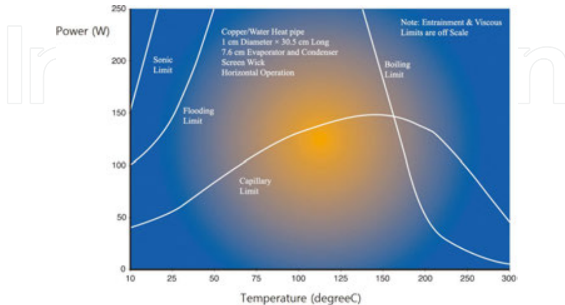
Figure 7. Performance limitations with respect to the temperature.
