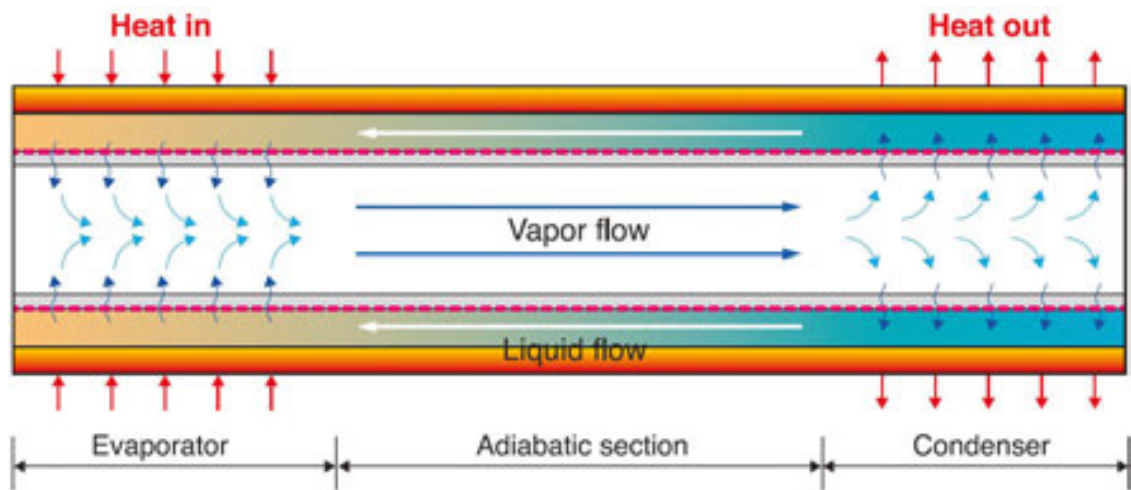
Figure 4. Working principle of heat pipe.
