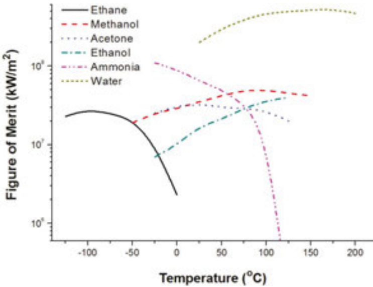
Figure 11. Figure of merit numbers of working fluids.
