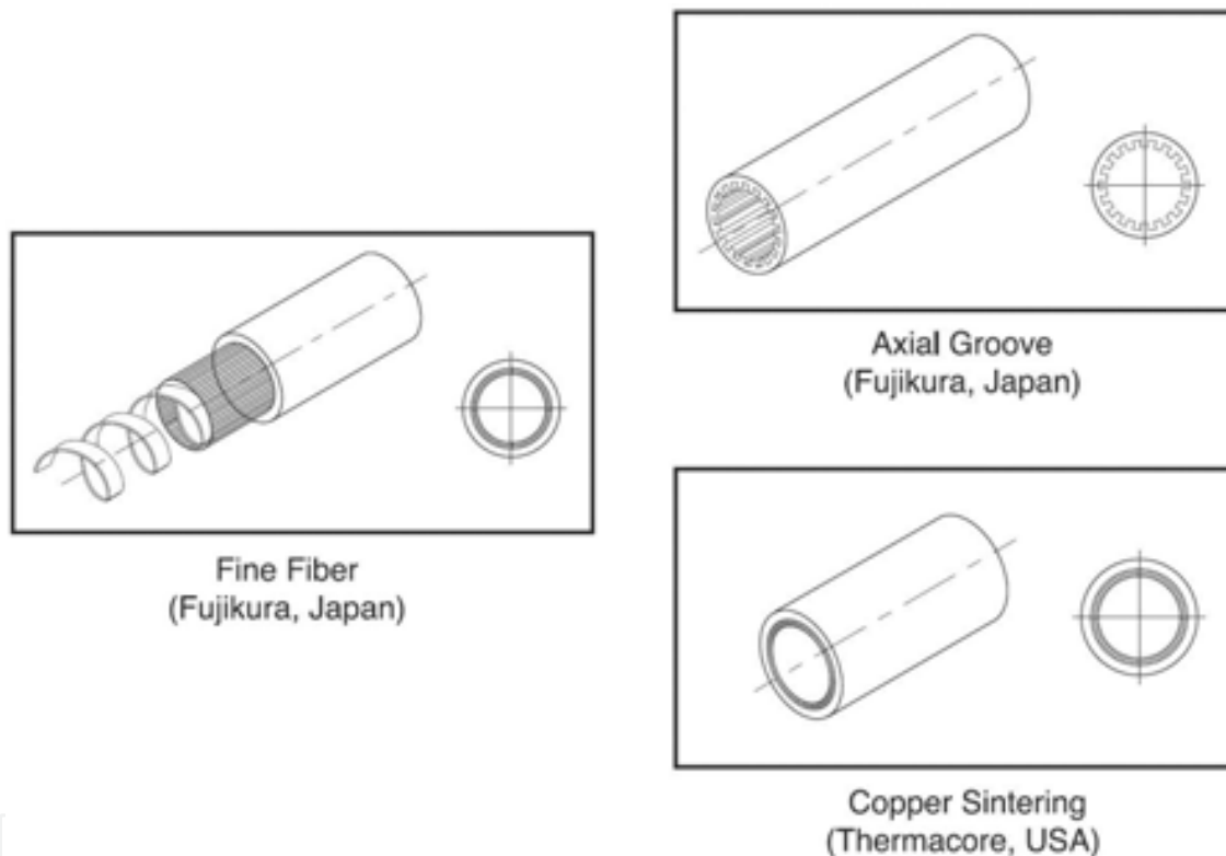
Figure 5. Typical wick structures.
