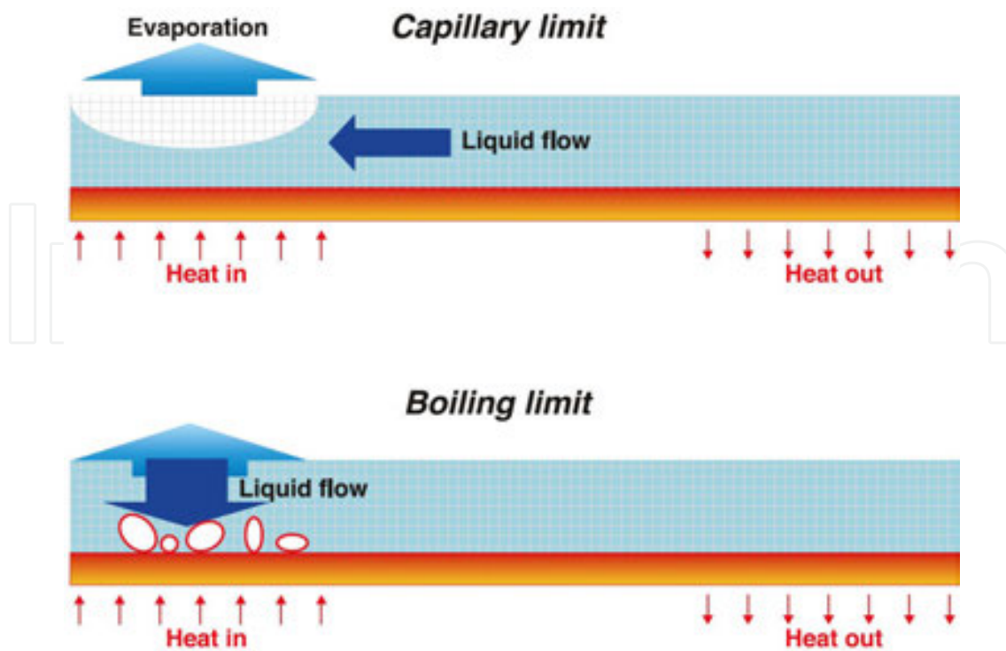
Figure 8. Capillary limit and boiling limit.
