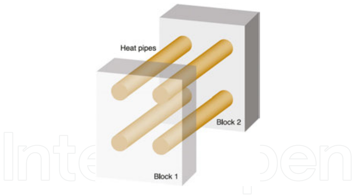
Figure 18. Block-to-block applications.
