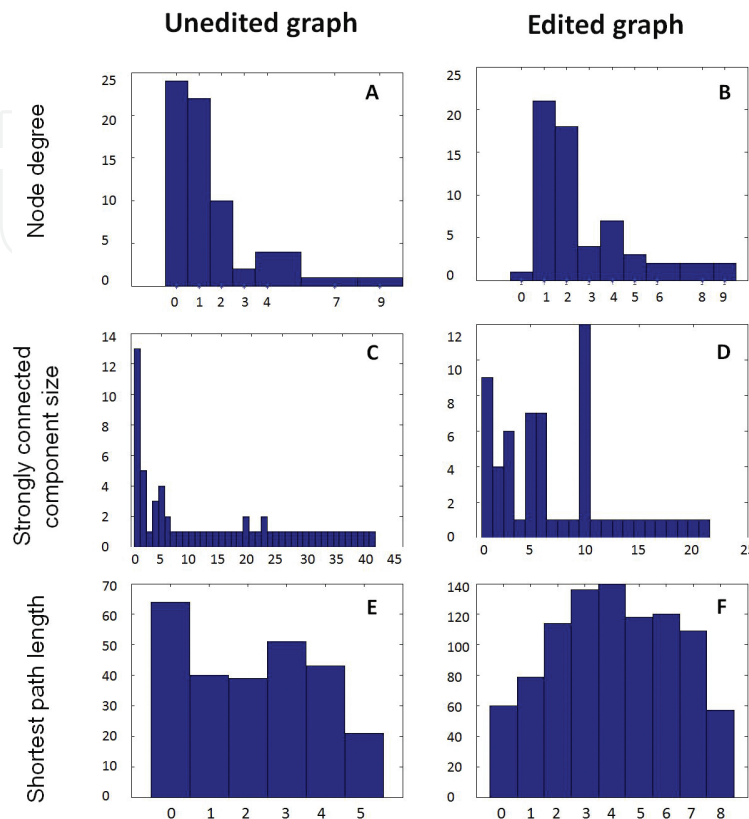
Figure 7. Graph characteristics of RIG-I-like signaling pathway after initial KGML parsing (unedited graph) and further editing to correct for missing nodes and edges (edited graph). (A and B) Node degree distributions; (C and D) the distributions of sizes of strongly connected components; and (E and F) the distribution of shortest path lengths.
