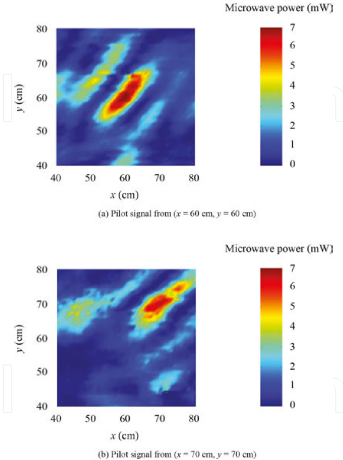
Figure 17. Microwave power distribution measured with the configuration in Figures 15 and 16 [20]. (a) Pilot signal from (x = 60 \text{ cm}, y = 60 \text{ cm}) . (b) Pilot signal from (x = 70 \text{ cm}, y = 70 \text{ cm}) .
