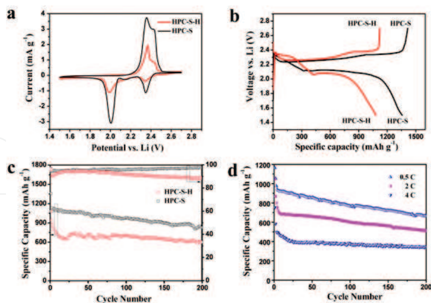
Figure 11. (a) Representative CVs of the HPCs-S-H and HPCs-S electrodes at a scan rate of 0.1 \text{ mV s}^{-1} between 1.5 and 2.7 V vs. Li/Li + . (b) Charge-discharge voltage profiles of HPCs-S-H and HPCs-S electrodes for the 1st cycle in the voltage range of 1.5–2.7 V at 0.2 C. (c) Capacity and Coulombic efficiency vs. cycle number of the HPCs-S-H and HPCs-S electrodes at 0.2 C. (d) Rate capability of the HPCs-S electrodes [28]
