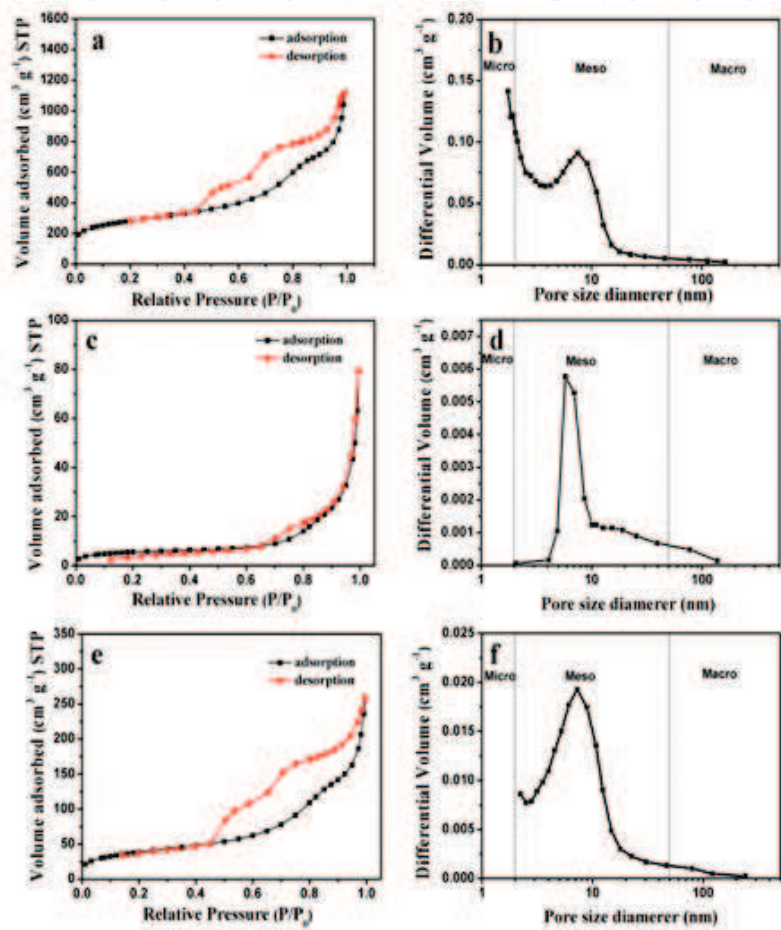
Figure 9. (a) N 2 adsorption-desorption and (b) the corresponding pore size distribution curve of HPCs composite; (c) N 2 adsorption-desorption and (d) the corresponding pore size distribution curve of HPCs-S-H composite; (e) N 2 adsorption-desorption and (f) the corresponding pore size distribution curve of HPCs-S composite [28].
