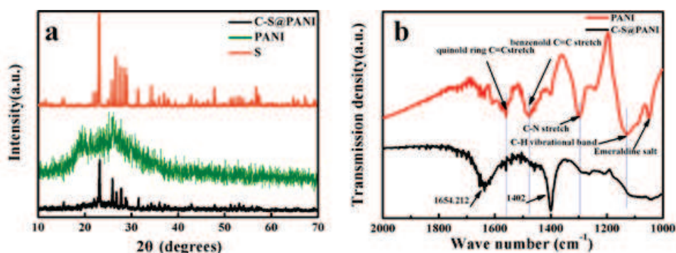
Figure 24. (a) XRD patterns of sublimed S, PANI and C-S@PANI composite 40% of sulfur, (b) FTIR spectra of the PANI and C-S@PANI composite [47].
