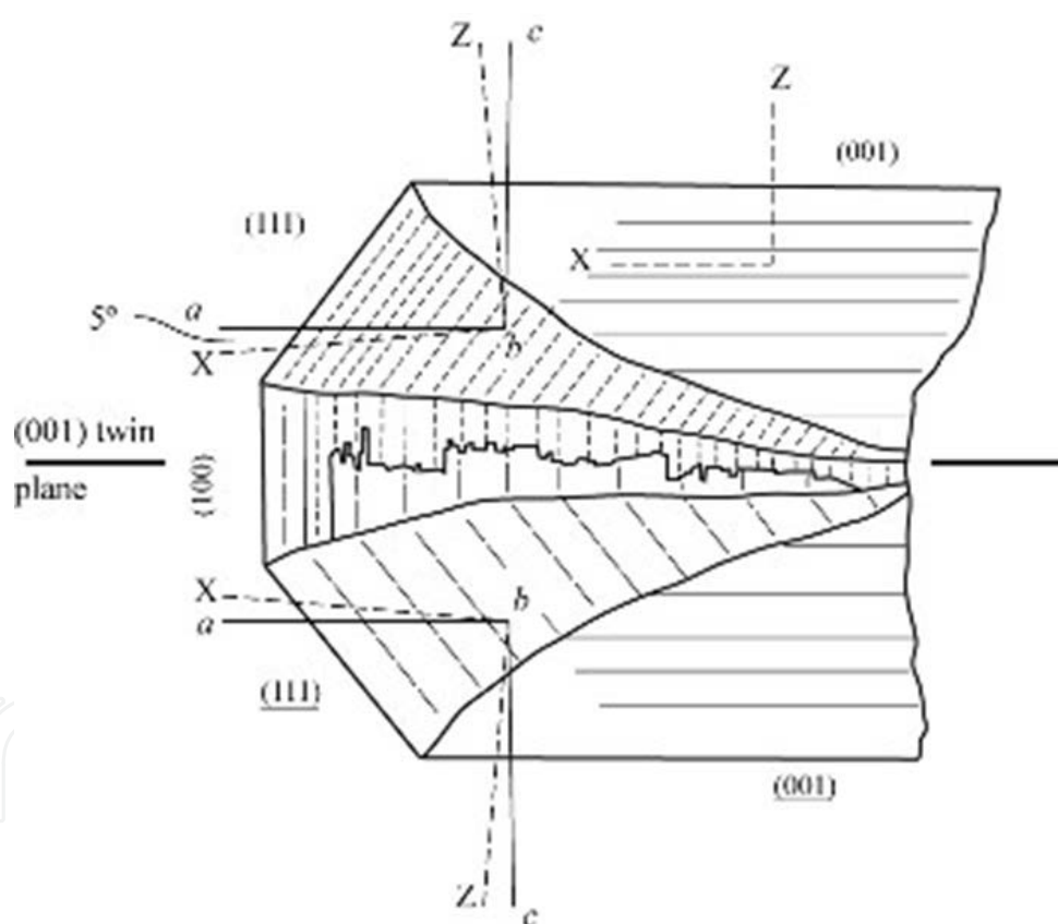
Figure 3. Crystallography of stilbite.
