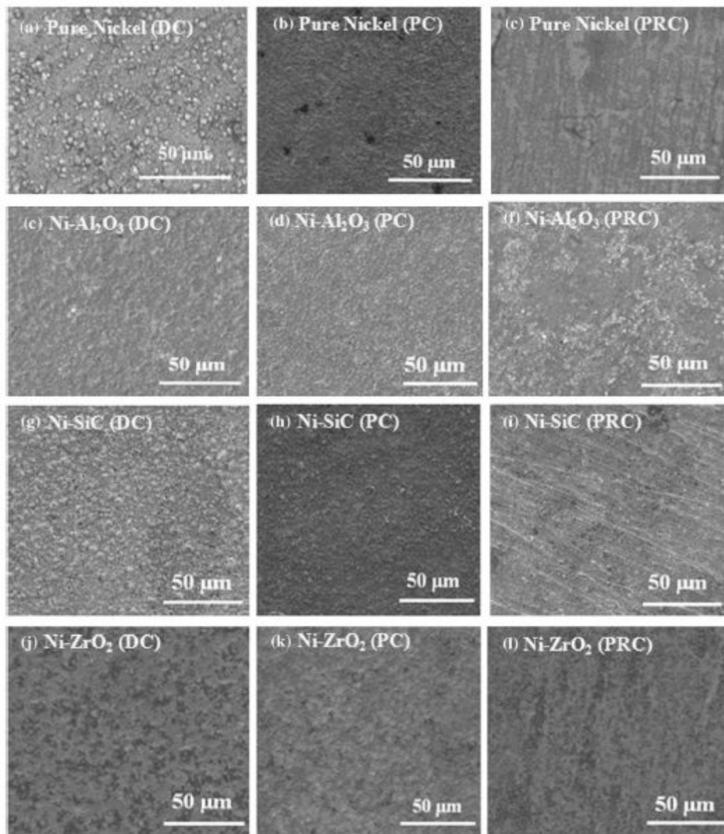
Figure 2. SEM micrographs of the plated samples [24]
