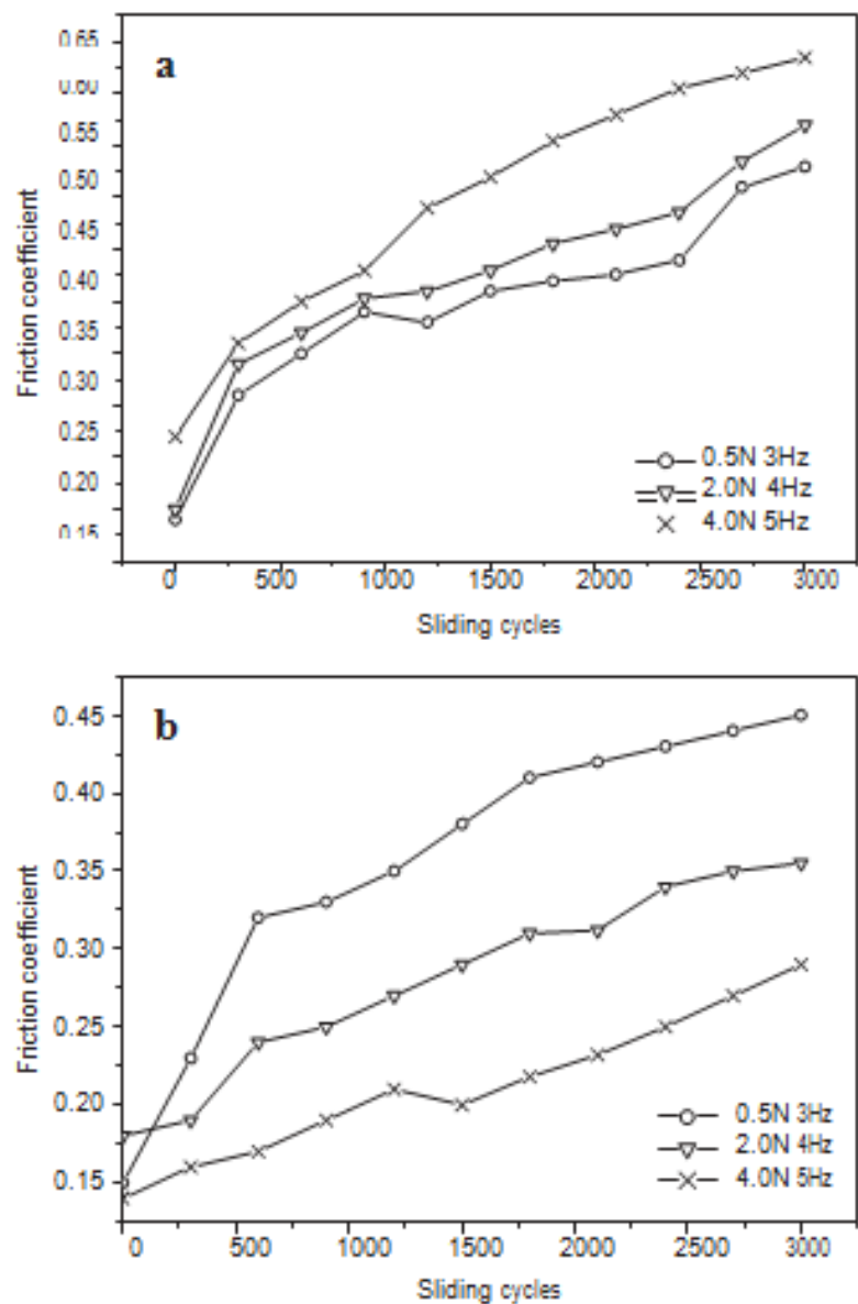
Figure 7. Friction coefficient of (a) Ni-Co alloy and (b) Ni-Co-CNT composite coating under different loads and sliding speeds [55]
