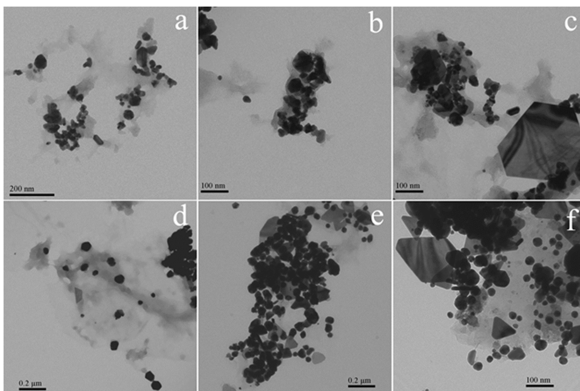
Figure 16. TEM images of gold nanoparticles by using different compounds to chloraurate ion ratio.
