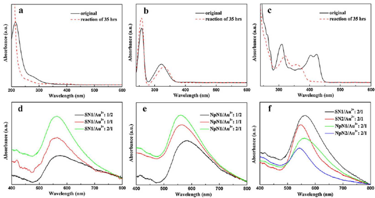
Figure 14. UV-Vis spectra of 0.1 mM \text{AuCl}_4^- ions and prepared gold nanostructures in aqueous solution.
