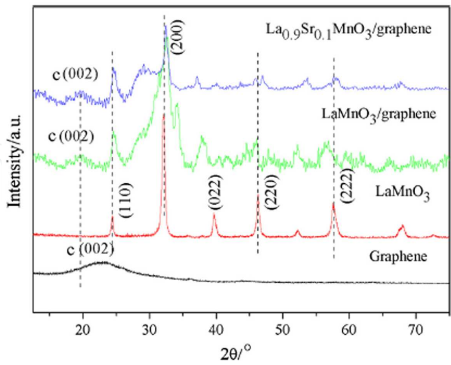
Figure 7. XRD pattern of graphene, LaMnO 3 , LaMnO 3 /graphene, and La 0.9 Sr 0.1 MnO 3 /graphene.
