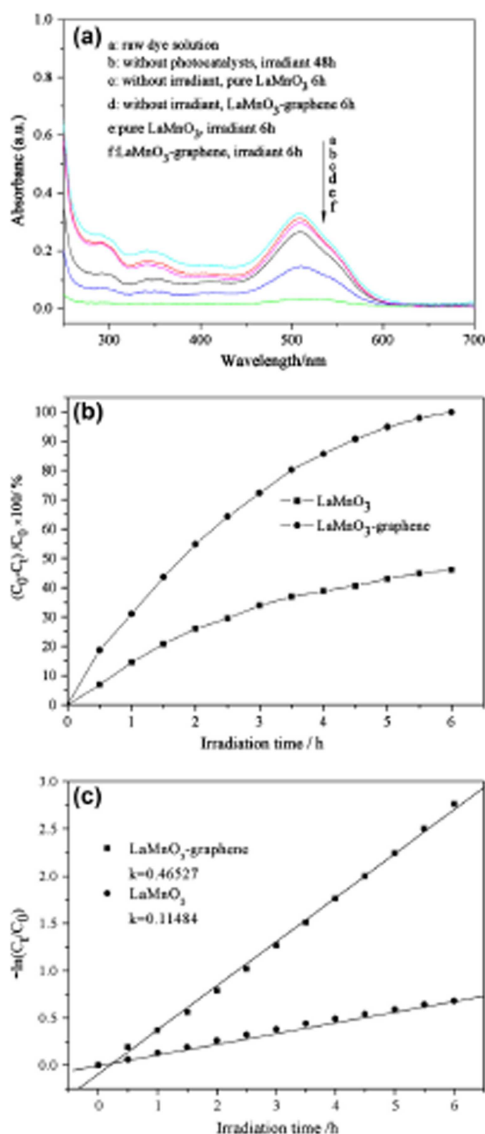
Figure 6. (a) UV-Vis spectral changes of the degradation of acid red A by \text{LaMnO}_3 -graphene and \text{LaMnO}_3 ; (b) photocatalytic activities of \text{LaMnO}_3 -graphene composite and \text{LaMnO}_3 ; (c) kinetics of photocatalytic degradation by the \text{LaMnO}_3 and \text{LaMnO}_3 -graphene.
