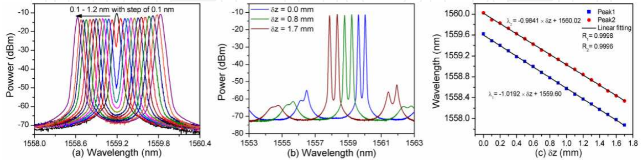
Figure 9. Experimental results of a tunable dual-wavelength fibre laser. (a) wavelength spacing is varied from 0.1 to 1.2 nm, (b) two wavelengths were simultaneously tuned by stretching the TCF, (c) two lasing wavelengths as a function of \delta z .
