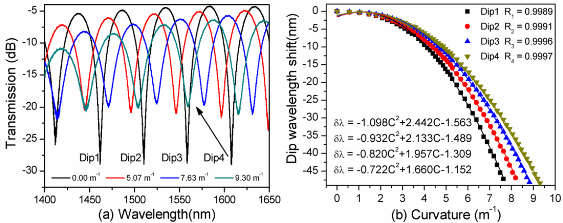
Figure 7. (a) Evolution of transmission spectra of the TCF-based filter, (b) dip wavelength shift against curvature.
