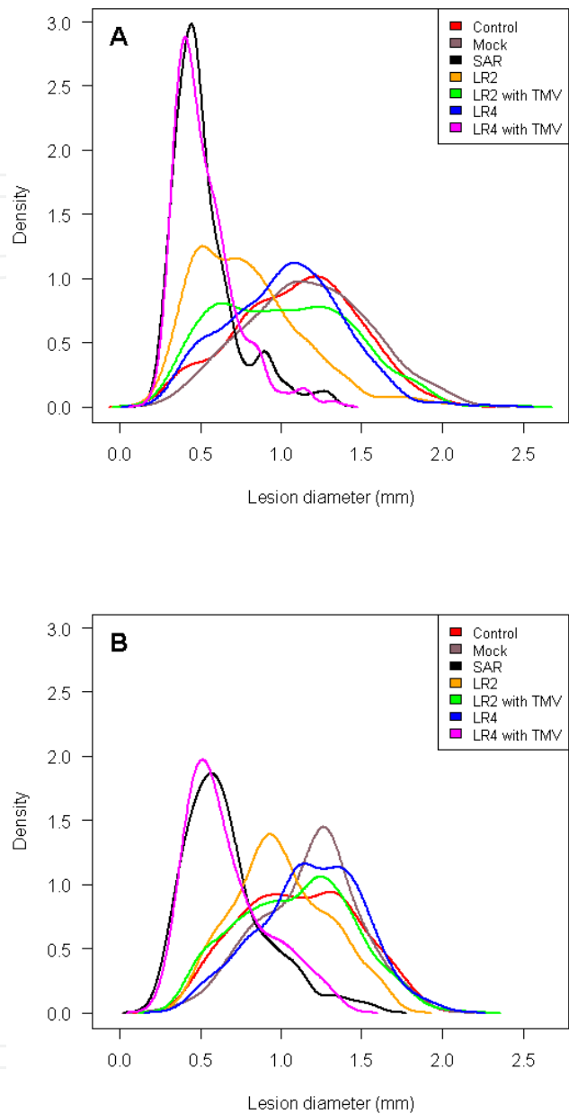
Figure 3. Kernel density estimation of TMV lesion size distribution on Nicotiana tabacum cv. Xanthi nc leaves at leaf level 5 (upper panel, A) and 6 (lower panel, B) after induction of systemic acquired resistance (SAR). For abbreviations and explanations of treatments see Fig. 2.
