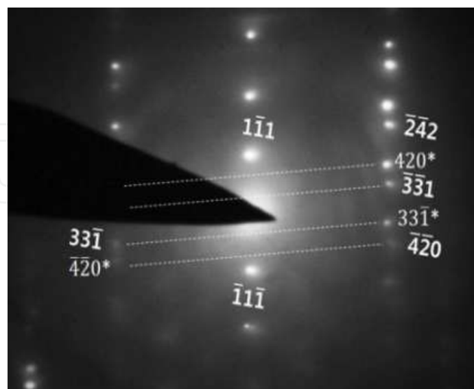
Figure 13. Twinning spots pattern from \gamma\text{Fe} with f.c.c crystal lattice which index matrix and twin spots with zone axis z = [\bar{1}23] , twinned on (1\bar{1}1) , hkl^* planes related to twin planes and hkl planes related to main reflected planes.
