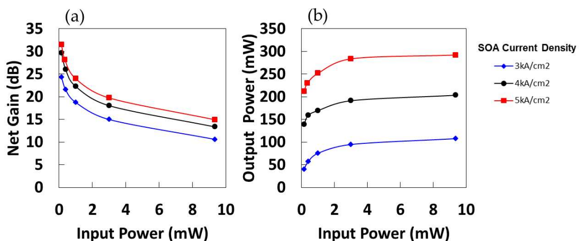
Figure 6. Net gain (left) and output power (right) obtained from the SOA (device A) as functions of CW input power for current densities of 3, 4, and 5 kA/cm 2 at an input wavelength of 404 nm.
