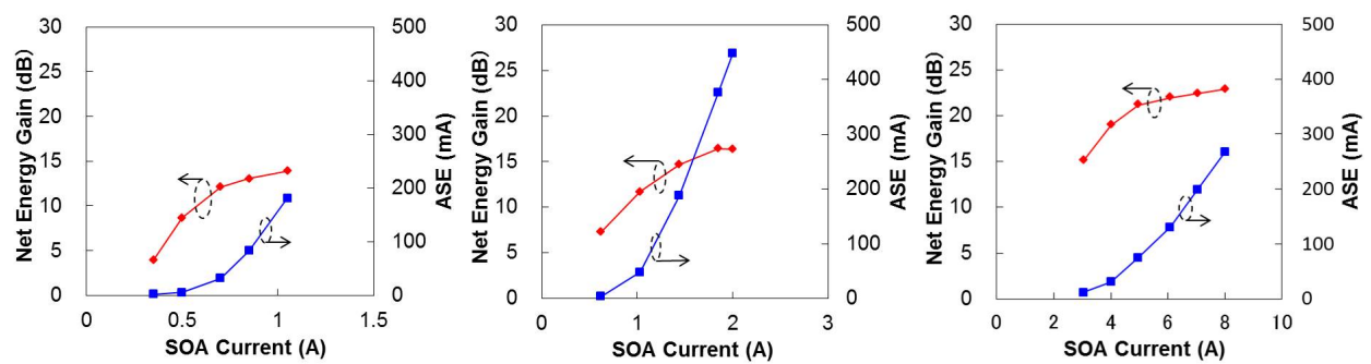
Figure 12. Net gain and ASE power values as functions of SOA current for devices B, C, and D.
