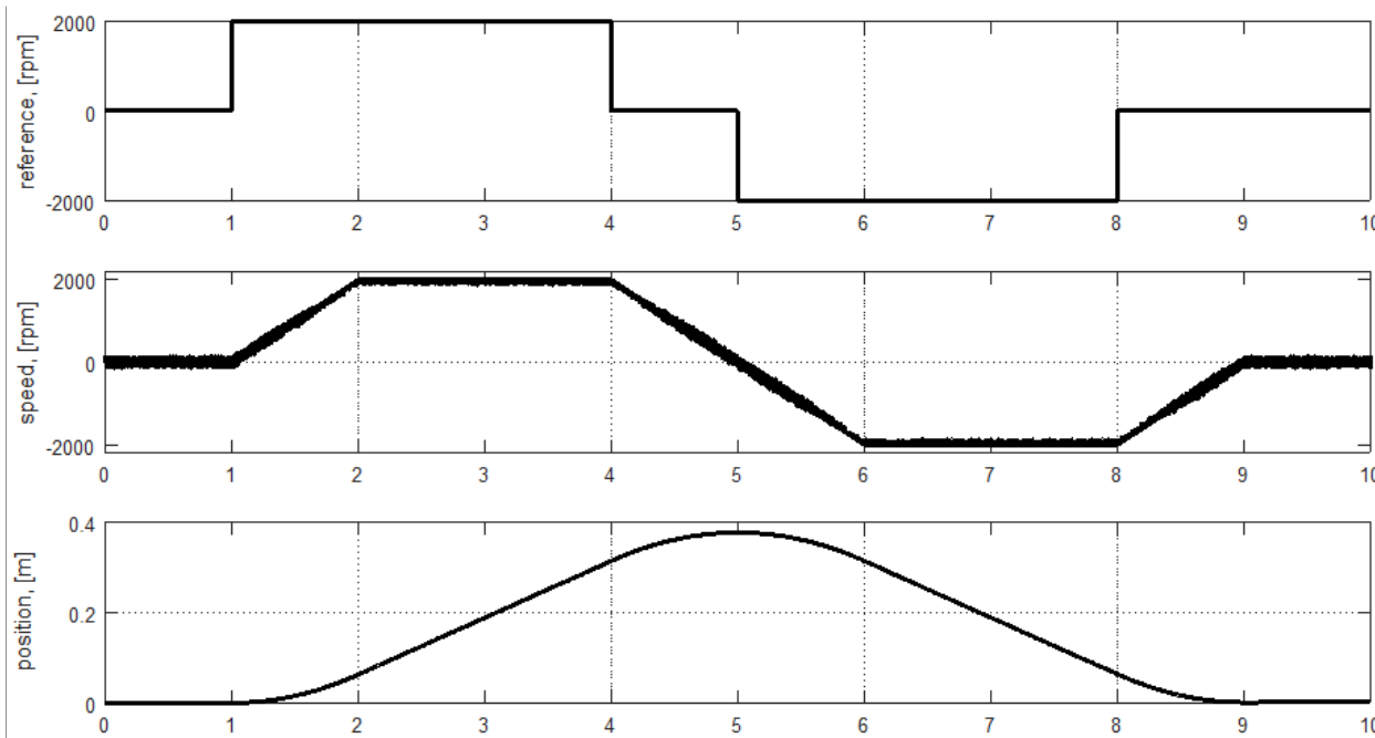
Figure 10. Simulation results of the DDH system: reference signal, motor speed and cylinder position.
