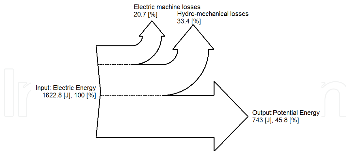
Figure 14. Measured Sankey diagram of the DDH with a motor speed of 400 rpm and a payload of 150 kg (the efficiency of the frequency converter is not included) [19].
