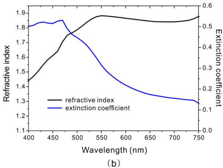
Figure 9. Refractive index and extinction coefficient of \text{CH}_3\text{NH}_3\text{PbI}_3 thin film [39].
