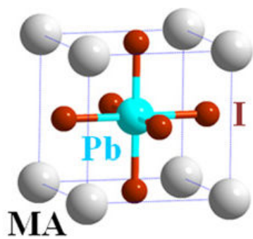
Figure 1. Perovskite structure. MA is [CH 3 NH 3 ] + [15].
