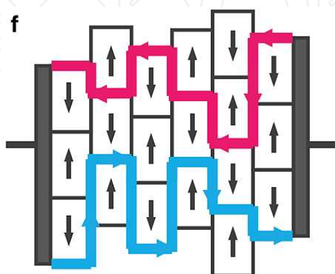
Figure 3. The propagation pathways of electrons and holes in \text{CH}_3\text{NH}_3\text{PbI}_3 [22].
