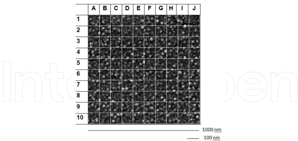
Figure 2. SEM observation of 0.5% Mn-doped ZnO NPs with a counting grid of 1000 × 1000 nm with small square sections of 100 × 100 nm to characterize NPs distribution and size.
