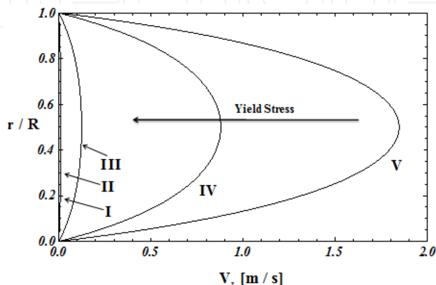
Figure 2. BMP model predictions for the velocity profile of pressure driven flow of a complex fluid with approximating from the no yield stress case (V) to the real yield stress case (I) in a circular pipe.
