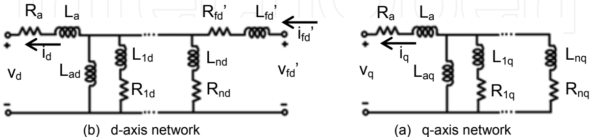
Figure 6: General d-q model equivalent circuit
