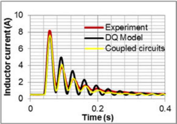
Figure 26. Field current when considering the saturation
