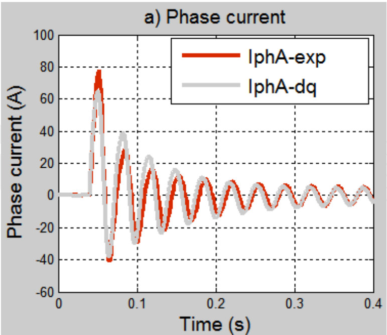
Figure 28. d-q model/experiment
