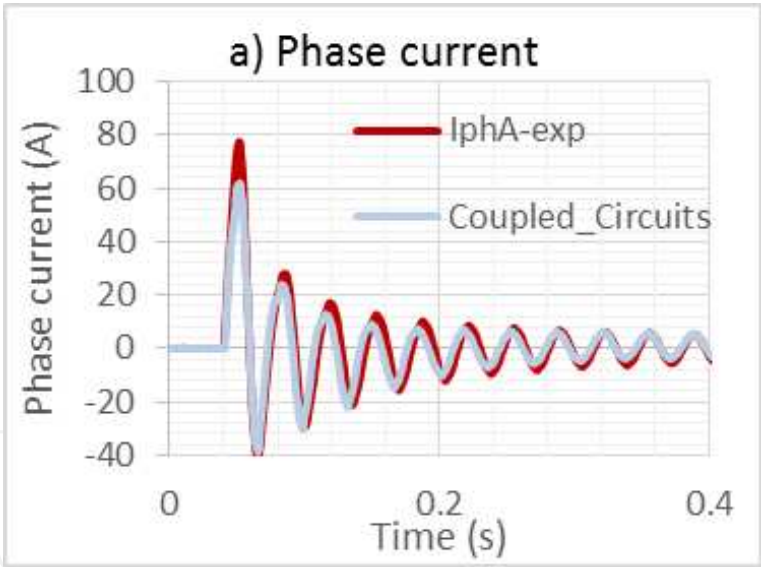
Figure 29. Coupled circuit/experiment
