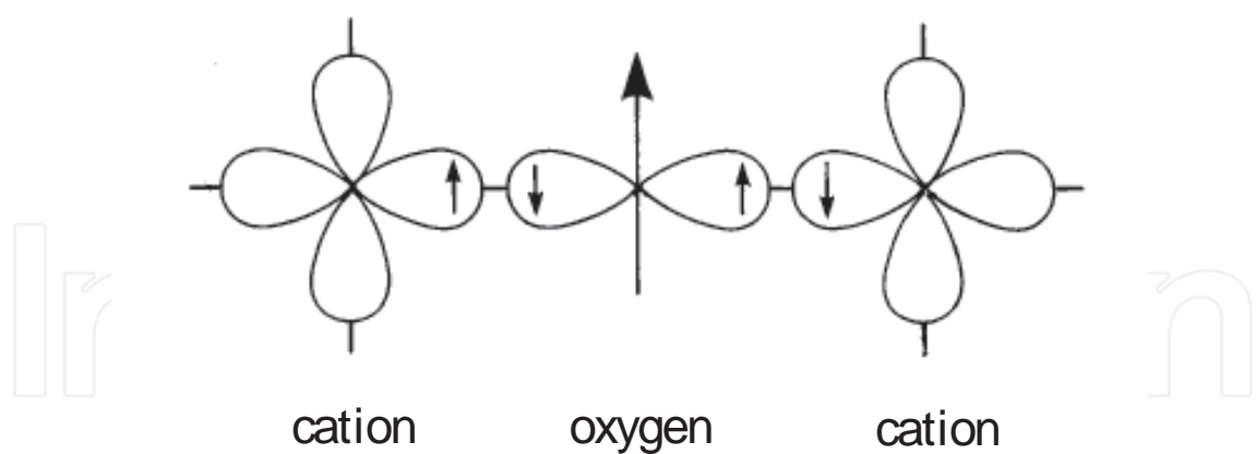
Figure 2. Superexchange interactions in ferrites.
