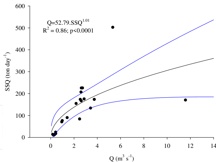
Figure 5. Suspended sediment rating curve of Capibaribe watershed.
