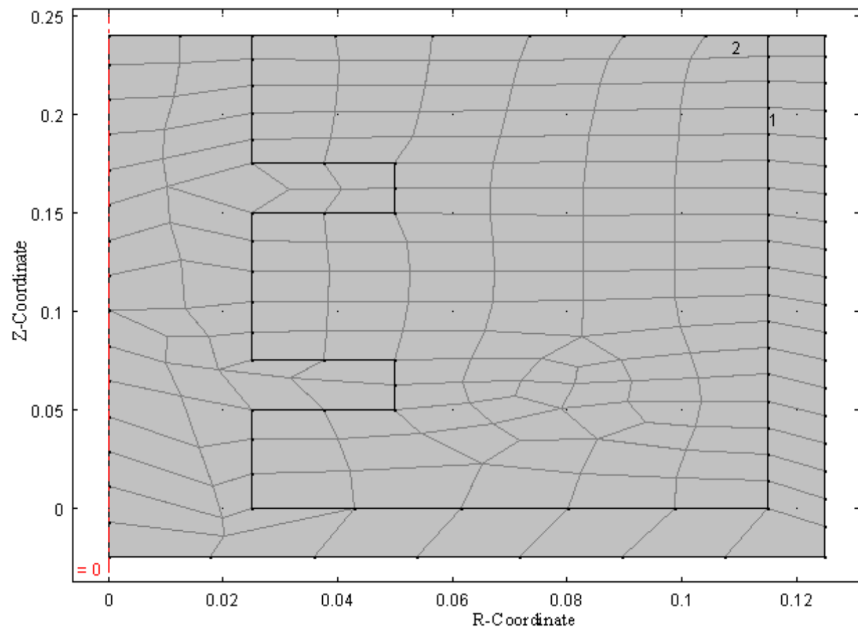
Figure 2. Computational Mesh.
