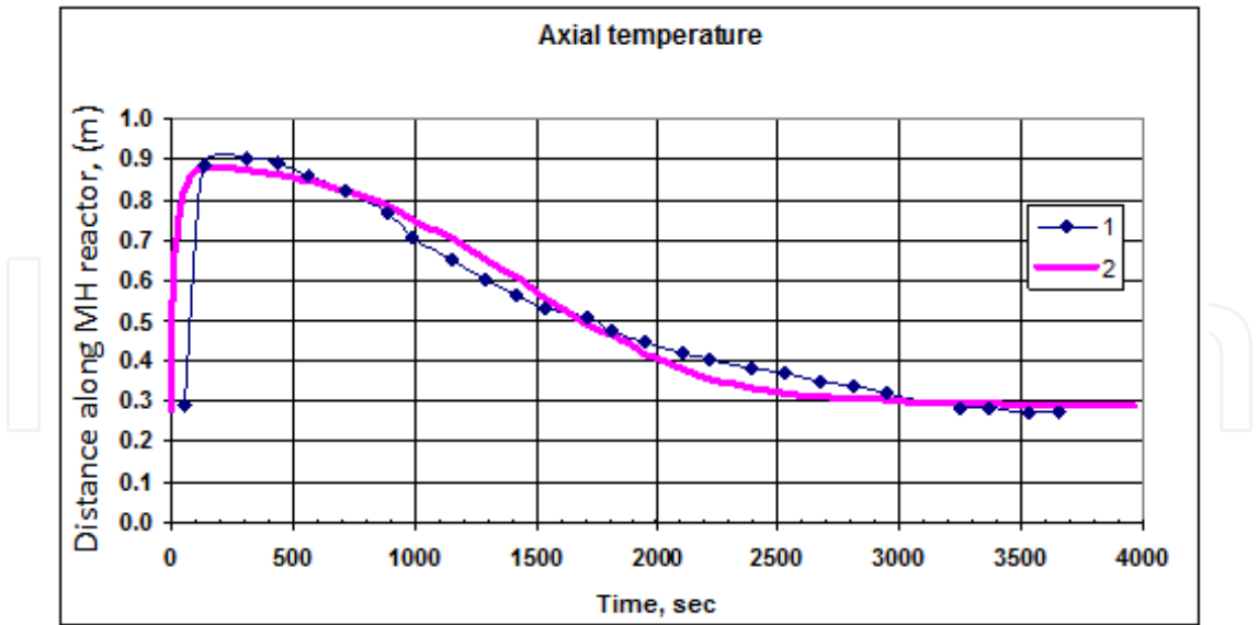
Figure 4. Axial temperature distribution in metal hydride reactor. 1 – Experiment (Jemni et. al. [3]-), 2 – calculations.
