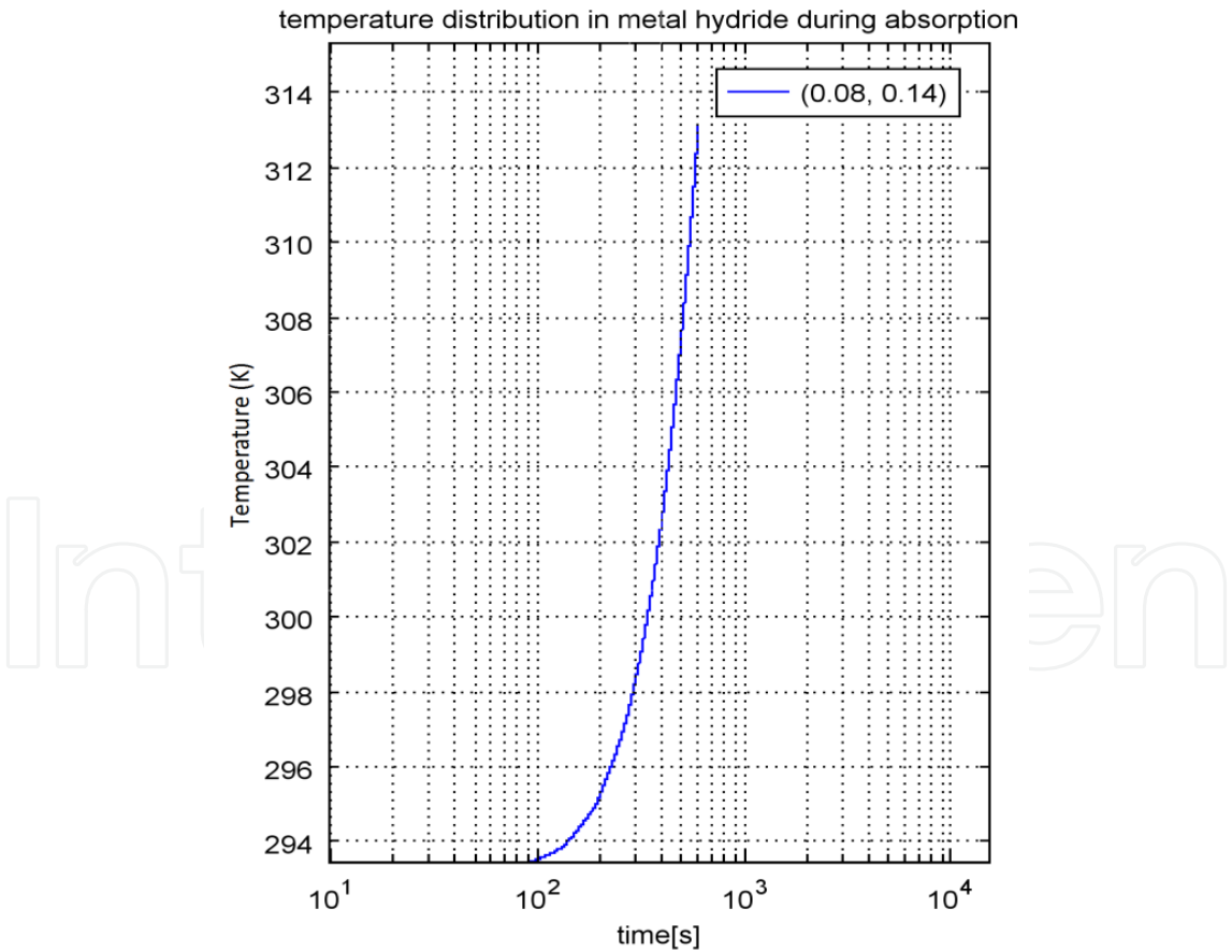
Figure 5. Time evolution of temperature in metal hydride reactor during absorption at point with coordinates [0.08, 0.14] during the 600-s period.
