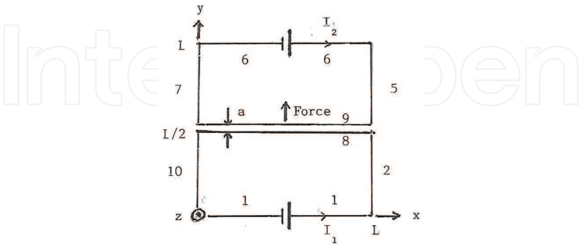
Figure 1. The configuration according to Ampère’s bridge used in order to realize a “two-infinite-parallel-conductor” circuit
