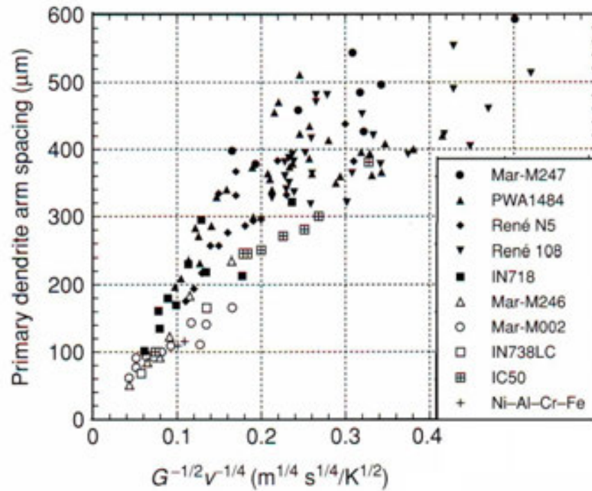
Figure 25. Some commercial superalloys' primary dendrite arm spacing with the combination G^{-1/2}v^{-1/4} , where G is the temperature gradient and v is the withdrawal velocity. Adapted from references [1, 47].
