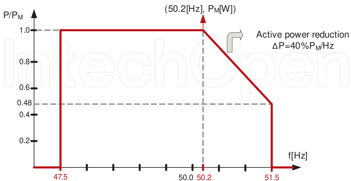
Figure 6. Standard characteristic P(f) for the generation unit.
