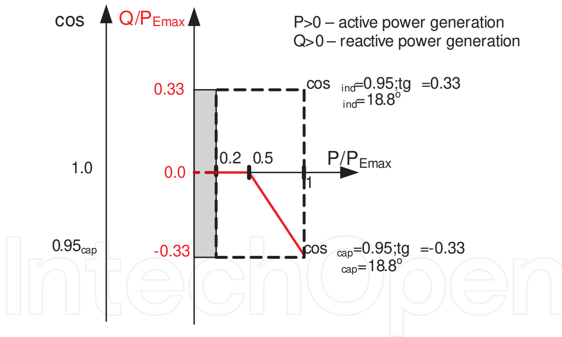
Figure 4. Standard characteristic \cos\varphi(P) for the generation unit within the range of maximum apparent power S_{E_{\max}} from 3,68 kVA to 13,8 kVA.
