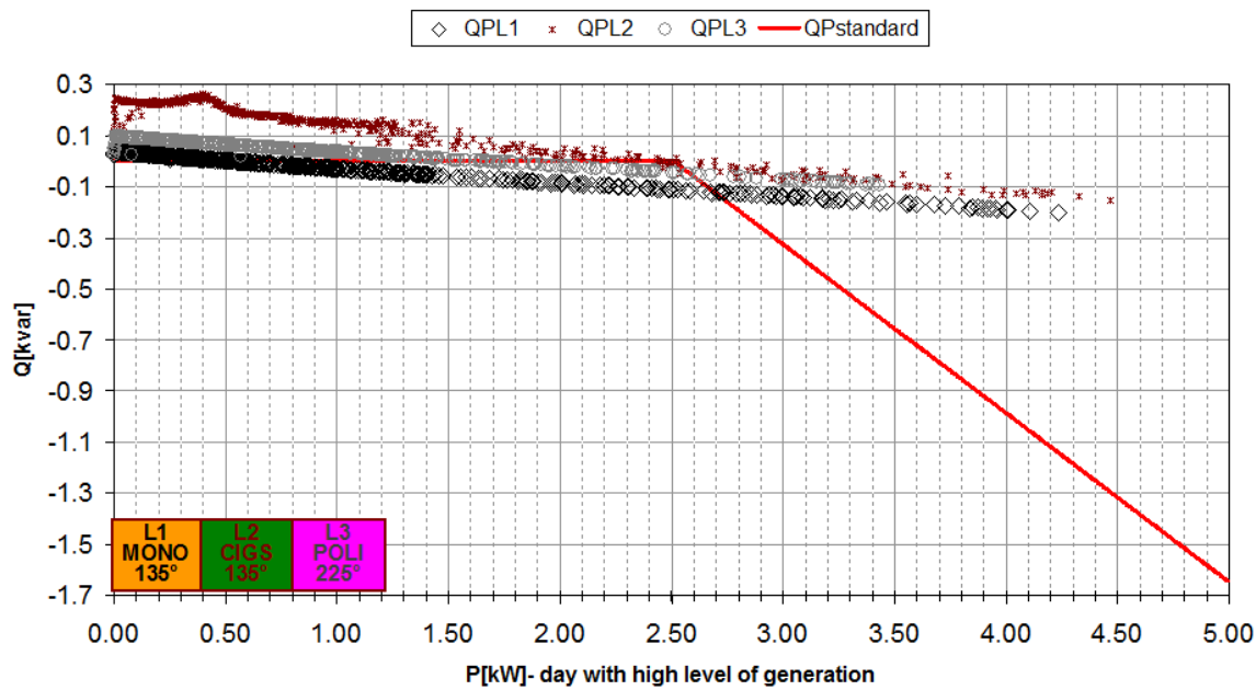
Figure 9. Comparison of reactive power regulation for particular PV subsystems in relation to the standard \cos\varphi (P) characteristic.
