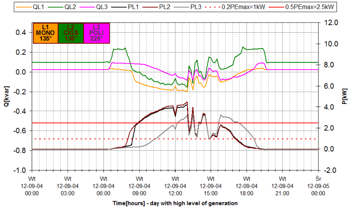
Figure 8. Reactive power regulation in relation to active power generation with characteristic coordintaes 0.2P_{Emax}=1 kW and 0.5P_{Emax}=2.5 kW.
