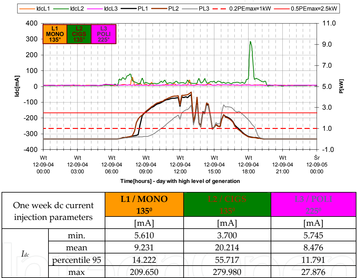
Figure 18. DC current injection in the PCC with reference to the PV subsystem’s active power generation and selected one-week data statistics.
