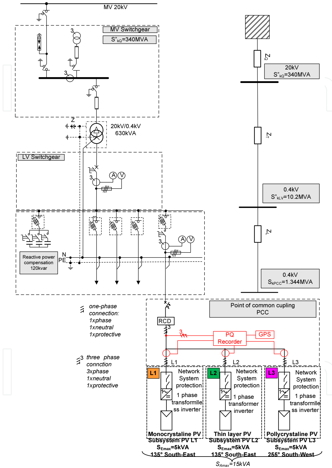
Figure 7. The diagram of interconnection of the investigated PV system with the LV network and its short circuit equivalent.
