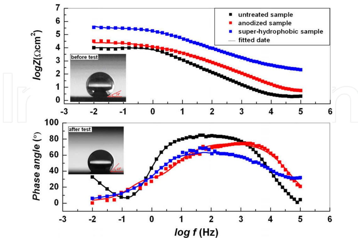
Figure 16. Bode plots of untreated, anodized, and super-hydrophobic samples after immersion in sterile seawater (32‰ NaCl, pH 8.02) for 24 h with the contact angle images of the super-hydrophobic surface before and after EIS test [94].
