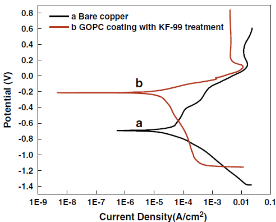
Figure 21. Tafel plots of (a) bare copper (b) GOPC coated copper after KF-99 treatment [113].
