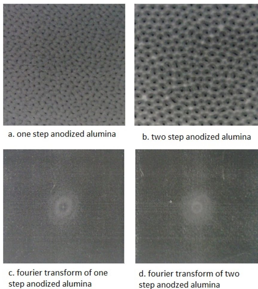
Figure 17. SEM images of one and two step anodization and their Fourier transforms.
