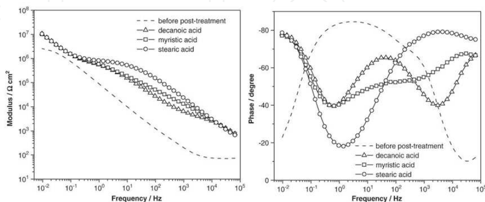
Figure 11. Bode plots of unsealed anodic layers obtained before or after post-treatment for 30 min 75 °C in pure molten acids (diagrams plotted after 2 h of immersion in 0.5 M \text{Na}_2\text{SO}_4 ) [90].
