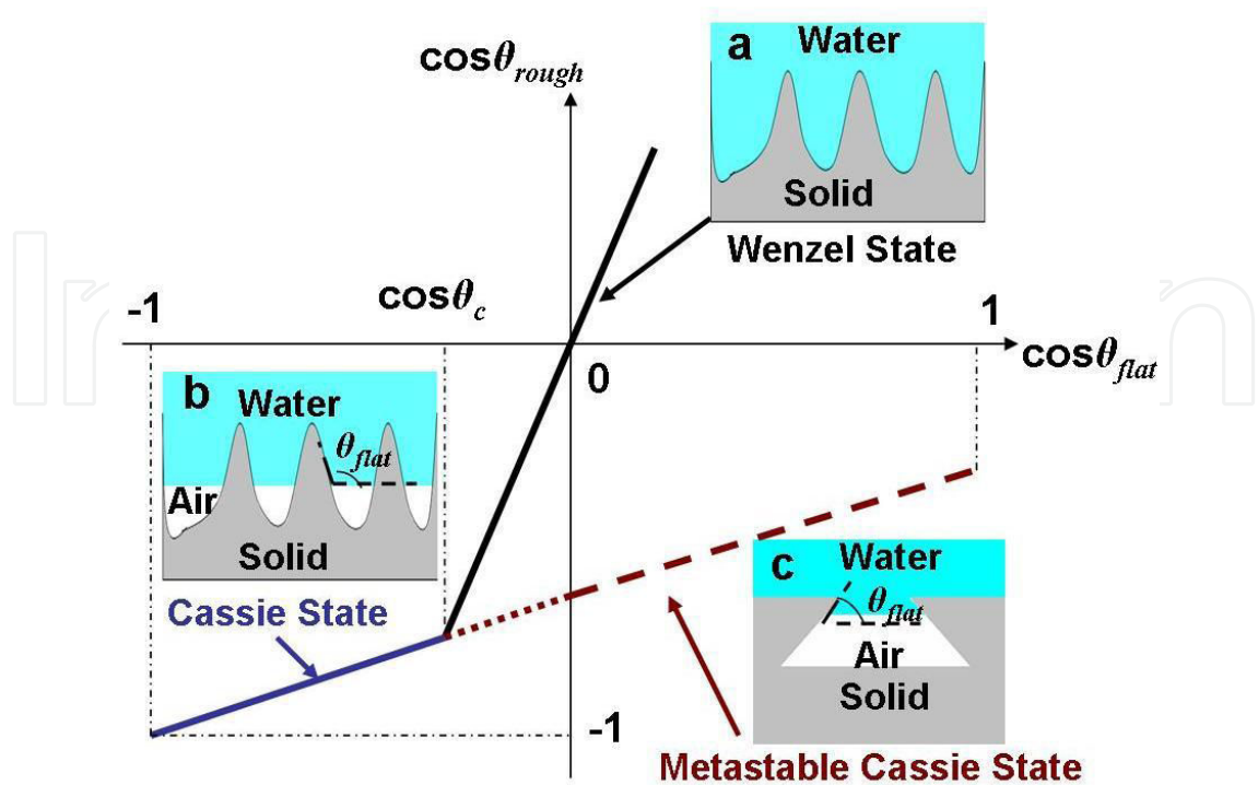
Figure 9. Relationship of rough \cos\theta with flat \cos\theta . The dotted and dashed lines correspond to the metastable Cassie state when \cos > 90^\circ flat \theta and the metastable Cassie state when \cos < 90^\circ flat \theta , respectively [58].
