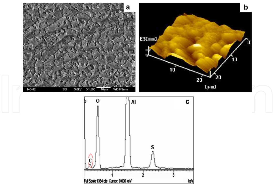
Figure 15. (a) SEM, (b) AFM, and (c) EDS of the super-hydrophobic aluminum surface [94].
