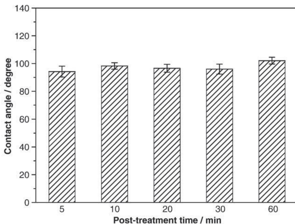
Figure 12. Contact angles measured on the surface of sealed anodic layers after post-treatment for 5-60 min at 75 °C in pure molten stearic acid [90].
