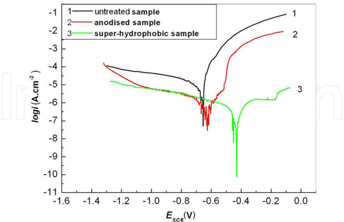
Figure 14. Potentiodynamic polarization curves of untreated, anodized, and super-hydrophobic samples for 24 h in sterile seawater at 2 mV s -1 [94].
