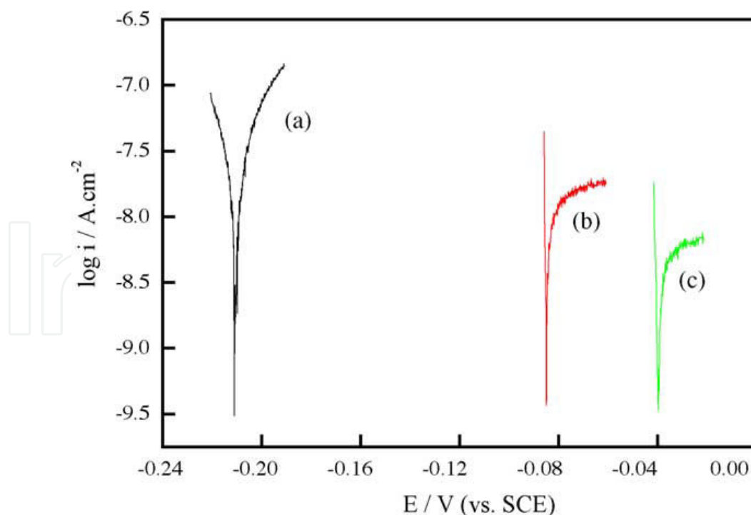
Figure 22. Polarization curves for bare 316L and films in oxygen-saturated Ringer solution. (a) Bare 316L; (b) \text{TiO}_2 / 316L coatings; (c) FSA/ \text{TiO}_2 / 316L coatings [125].
