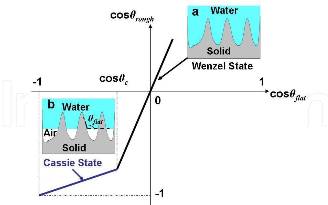
Figure 8. Relationship of \cos \theta_{\text{rough}} with \cos \theta_{\text{flat}} . The black solid and blue solid lines correspond to the Wenzel state and the Cassie state, respectively [58].
