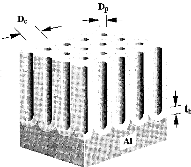
Figure 18. Ideal hexagonal “alumite” or PTF. Metallic Al, on the bottom, is covered by an impervious “barrier” oxide of thickness t_b and then by a hexagonal array of pores of diameter D_p , with a cell (repeat) distance D_c [101].
