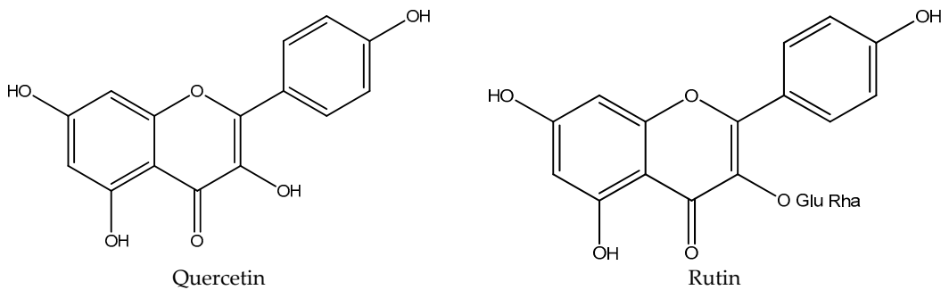
Figure 2. Chemical structures of flavonoids in investigated thyme extracts (Glu = glucose, Rha = rhamnose)
