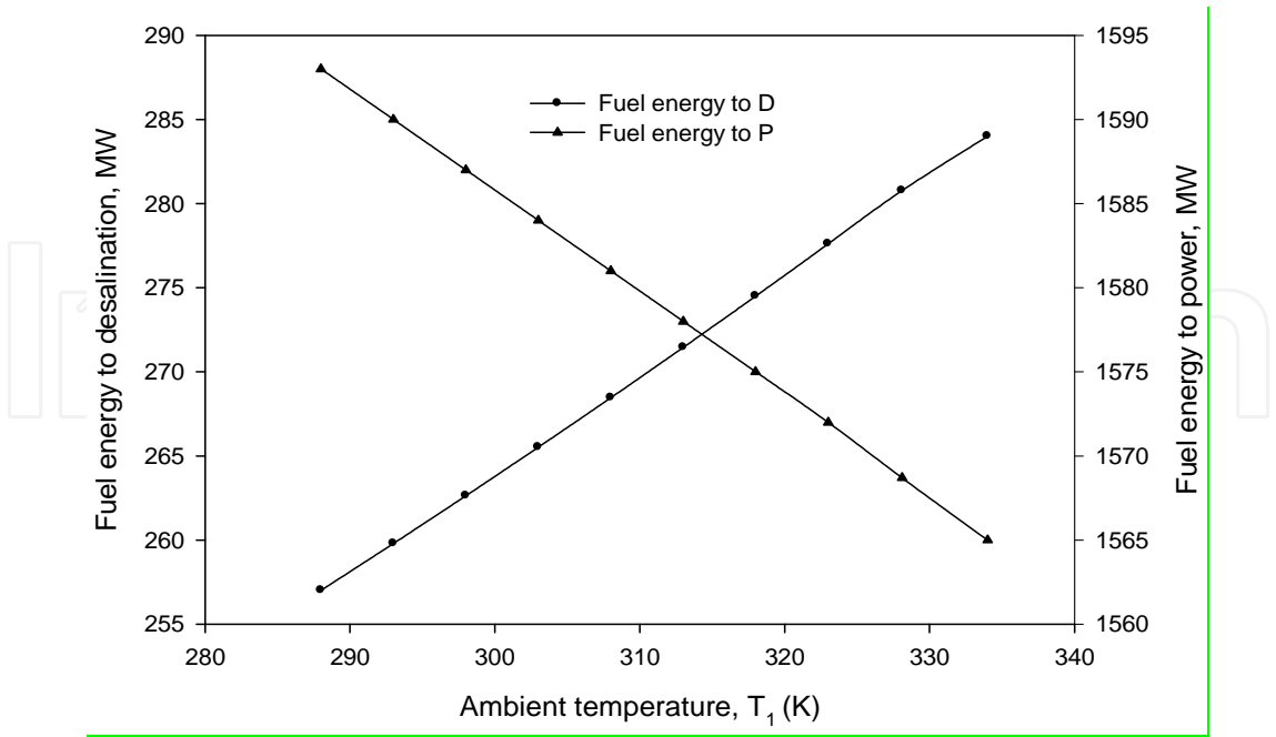
Figure 31. The effect of air ambient temperature to fuel allocation between the electric power and desalinated seawater production
