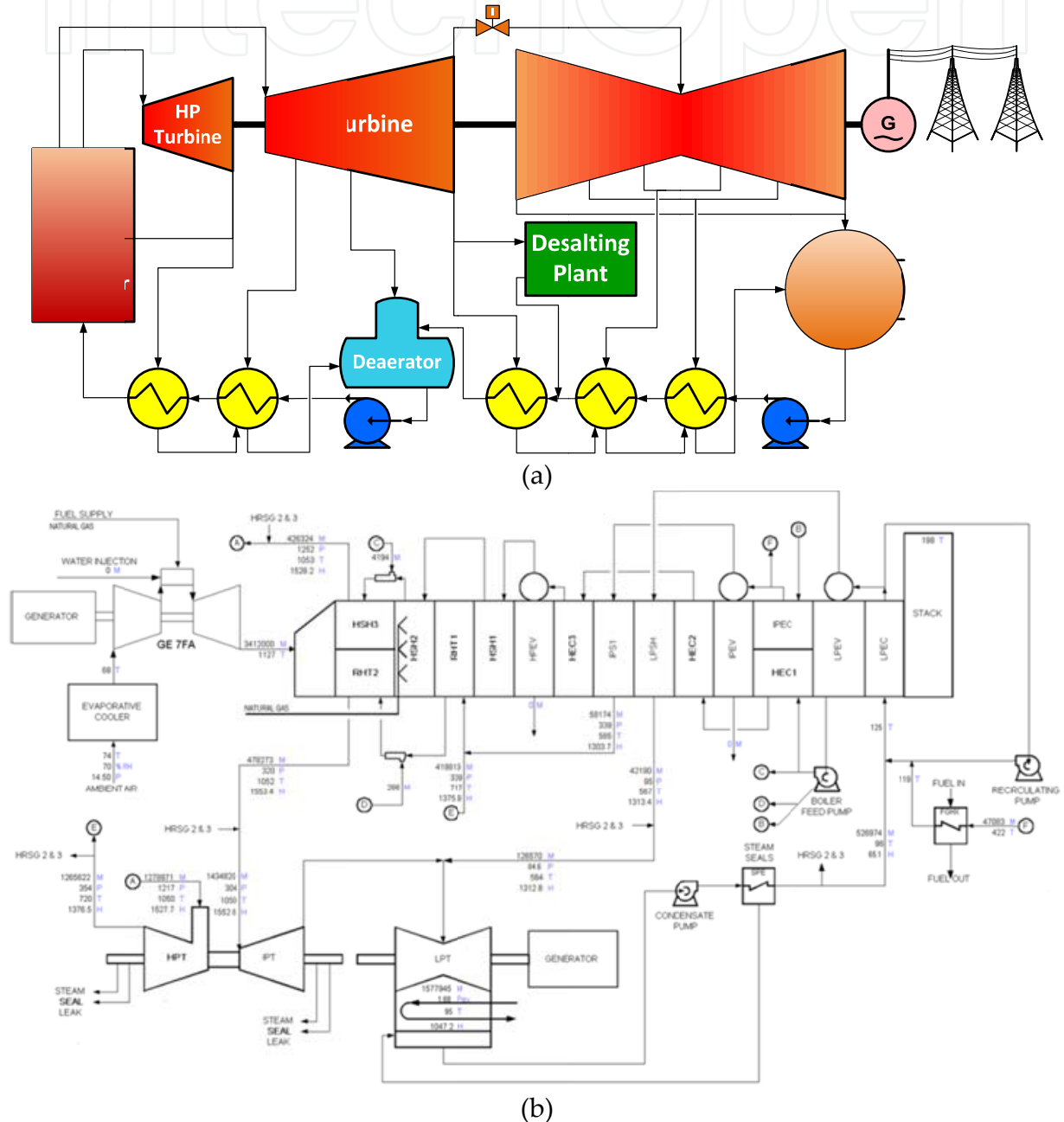
Figure 19. a: Conventional steam power plant operated by fuel-operated steam generator. b: Combined GTCC using 3 GT, 3 HRSG, and one steam turbine [5]
