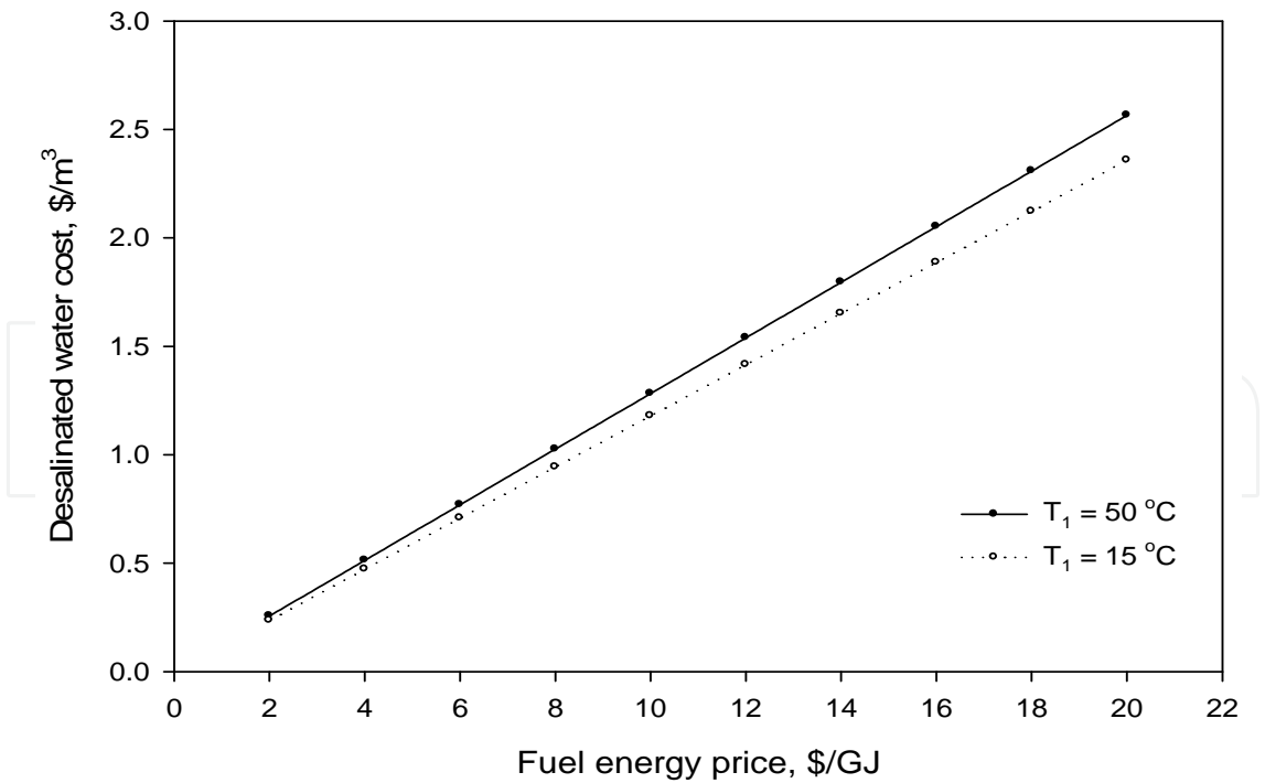
Figure 38. The effect of fuel energy price on the desalinated water cost at different ambient temperatures
