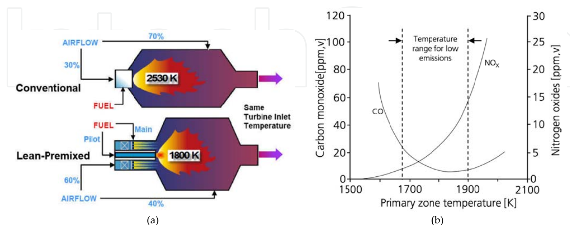
Figure 13. a: Schematic of a conventional and a lean-premix combustor [20] b: Primary zone temperature influence on \text{NO}_x and CO emissions [8]
