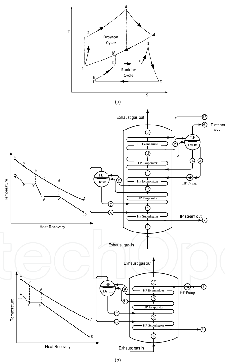
Figure 17. a: Upper GT turbine cycle (Brayton) and bottom Rankine steam cycle. b: HRSG of dual pressure in the middle and single pressure at the bottom steam stages and their temperature distribution [20]
