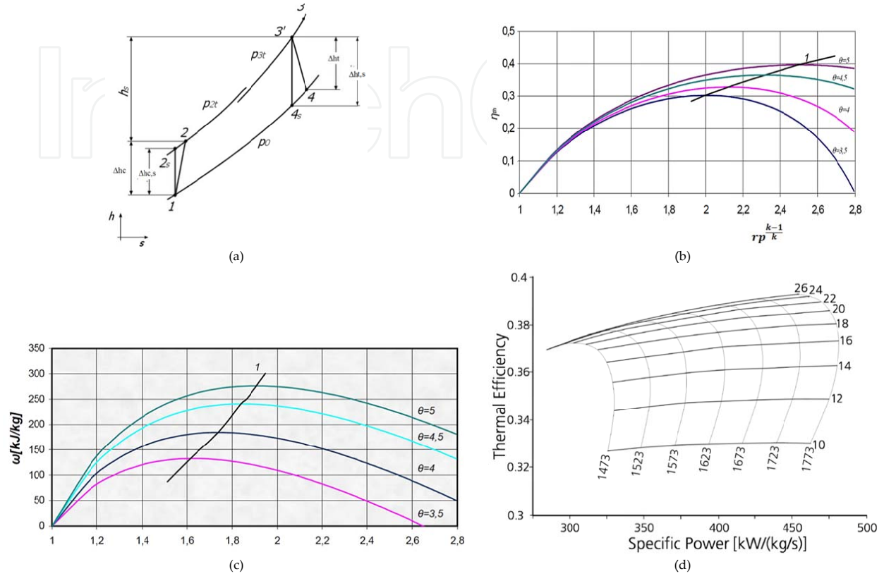
Figure 6. a: Enthalpy-entropy ( h - s ) diagram for ideal and practical gas turbine cycle [7] b: Dependence of the thermal efficiency \eta_{th} of the cycle on the parameters rp , k , and \theta for \eta_{t,is} = 0.88 and \eta_{c,is} = 0.86 . Line 1 joins points of maximum efficiency for each curve [7] c: Dependence of the specific work of the cycle on the parameters \pi , \kappa , and \theta for \eta_T = 0.88 and \eta_C = 0.86 . Line 1 joins points of maximum specific work for each curve [7] d: Thermal efficiency vs specific power for varying pressure ratios (10–26) and combustor outlet temperature (1,473–1,773 K) for a gas turbine [8]
