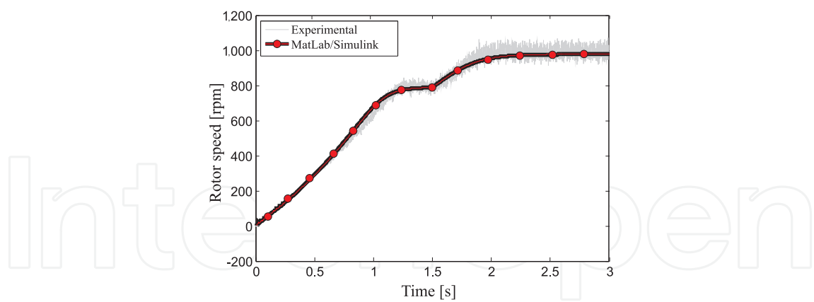
Figure 7. Transient rotor speed evolution
