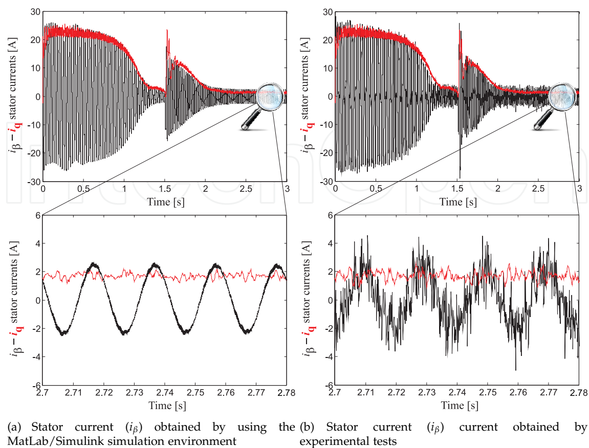
Figure 6. Stator current start-up characteristics
