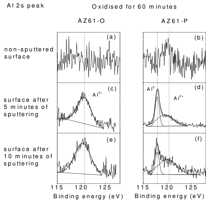
Figure 10. Variation of the Al2s high-resolution peak obtained by XPS on the surface of the AZ61-O and AZ61-P oxidised for 60 minutes as a function of the time of sputtering (figure adapted from [45] and [46]).
