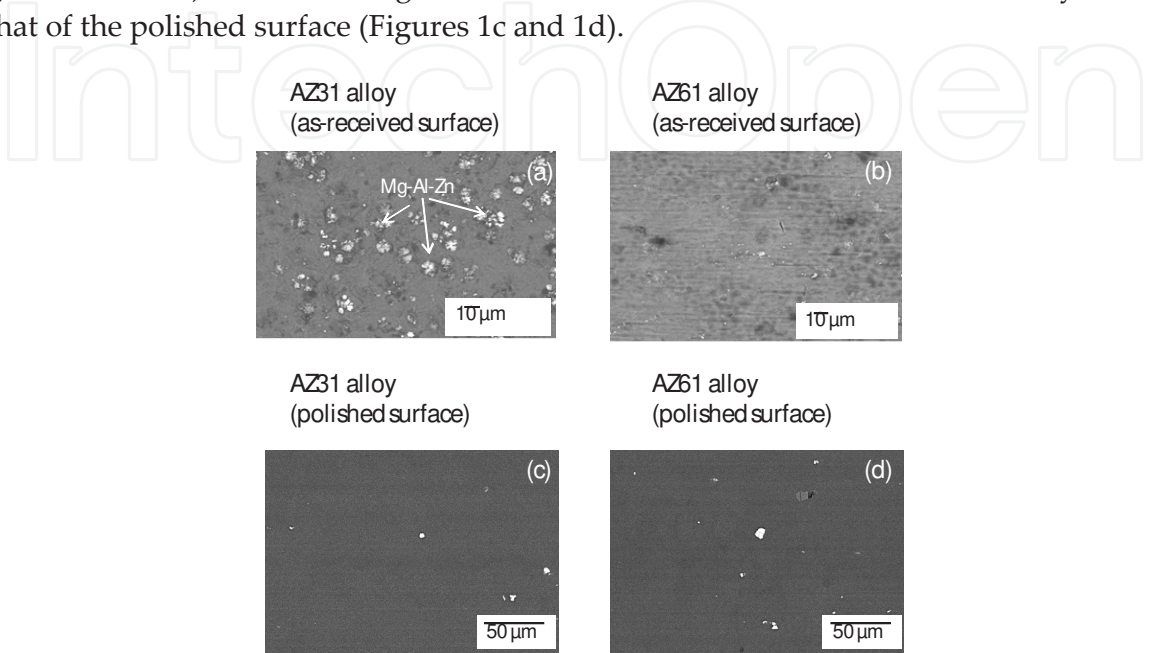
Figure 1. (a, b) SEM morphologies of the surfaces in the AZ31-O and AZ61-O and (c, d) AZ31-P and AZ61-P specimens (figure adapted from [45] and [46]).
