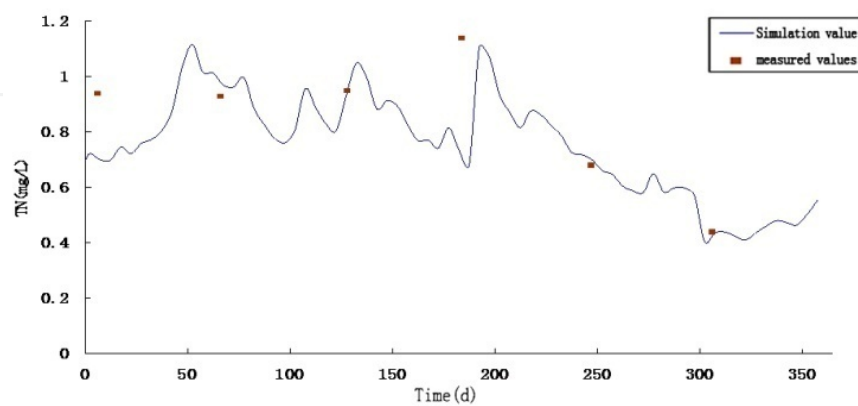
Figure 27. The verification chart for Tangling Lake TN.
