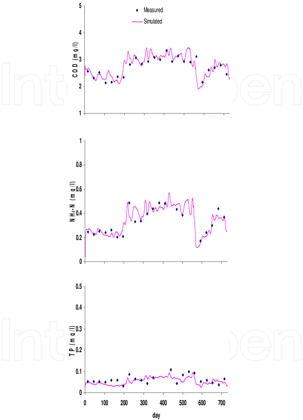
Figure 13. Water-quality validation results of typical control cross-section 3 (calculated and measured concentration of COD Miv , NH 3 -N and TP).
