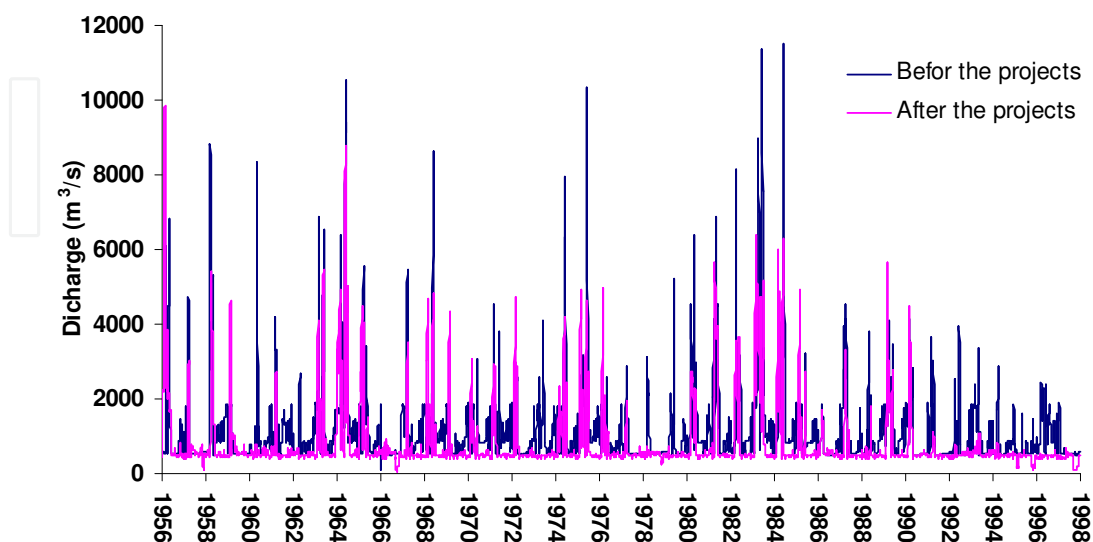
Figure 14. Calculated daily discharge of section 1 before/after the projects.
