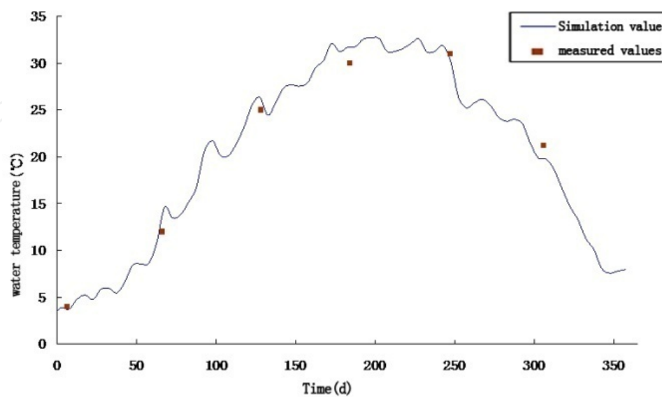
Figure 21. Verification chart for Miao Lake temperature.
