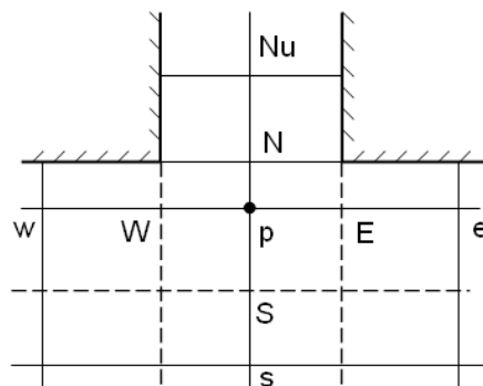
Figure 1. One-dimensional and two-dimensional models of connection.
