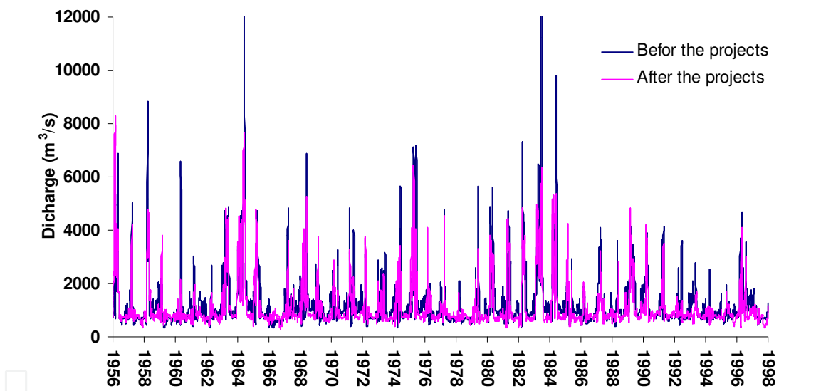
Figure 16. Calculated daily discharge of section 13 before/after the projects.
