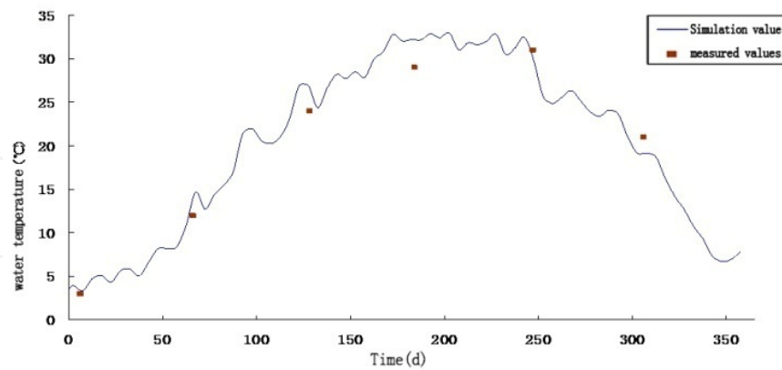
Figure 25. Verification chart for Tangling Lake temperature.
