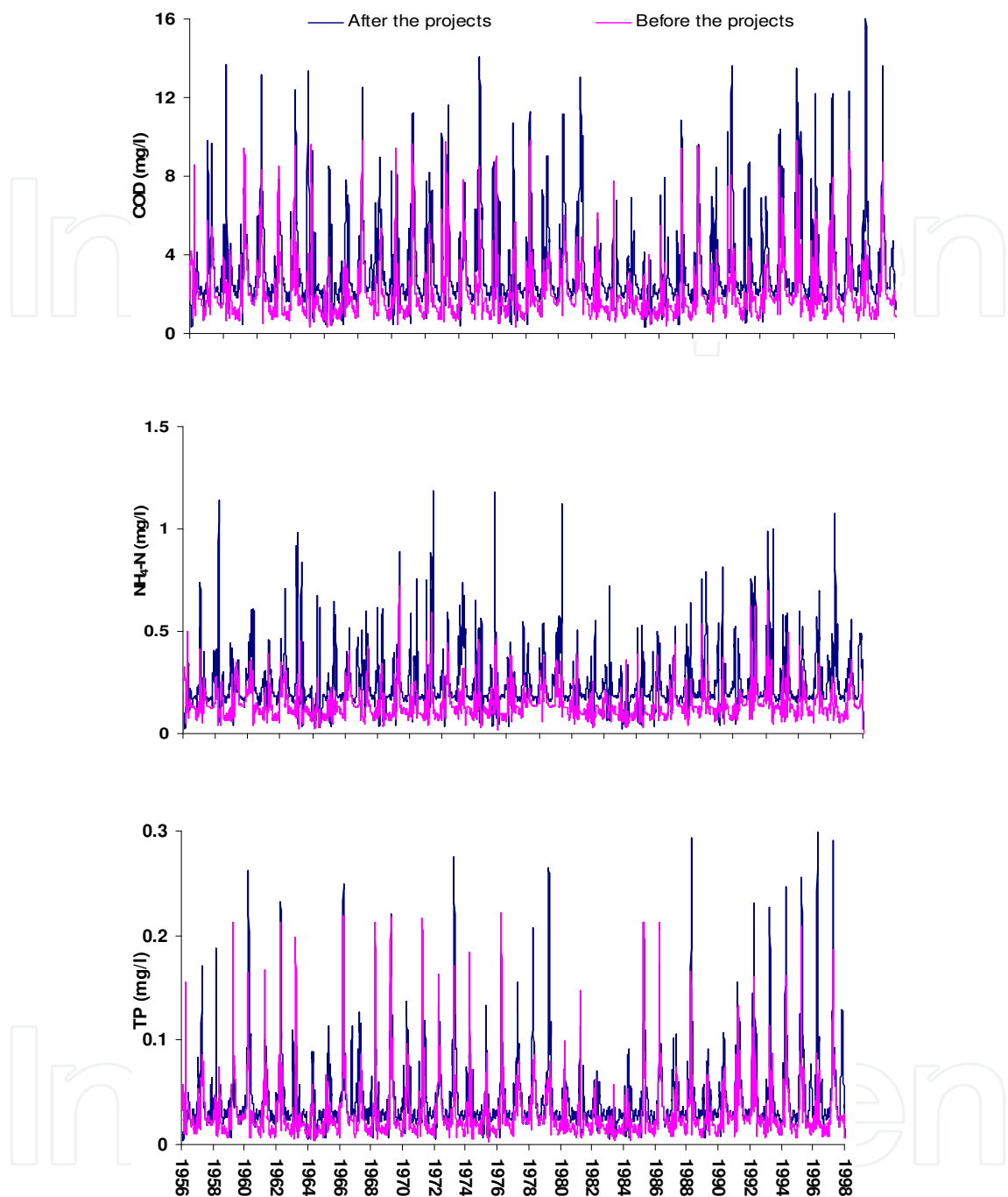
Figure 17. Calculated daily concentrations of COD, NH 3 -N and TP of section 4 before/after the projects
