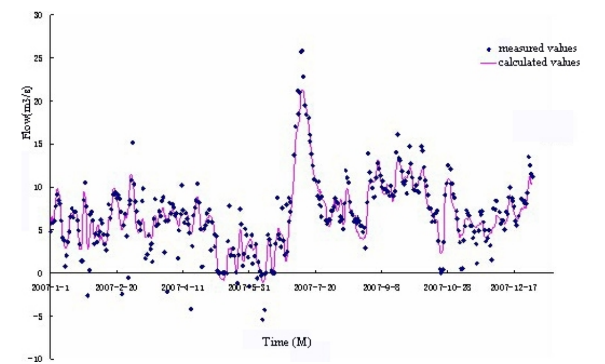
Figure 6. Flow verification of Caoqiao section.
