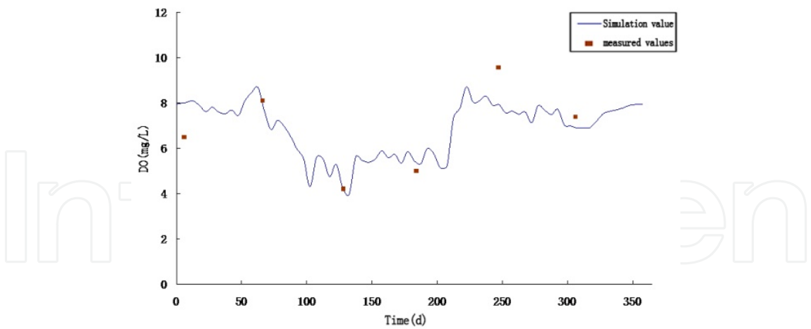
Figure 22. Verification chart for Miao Lake DO.
