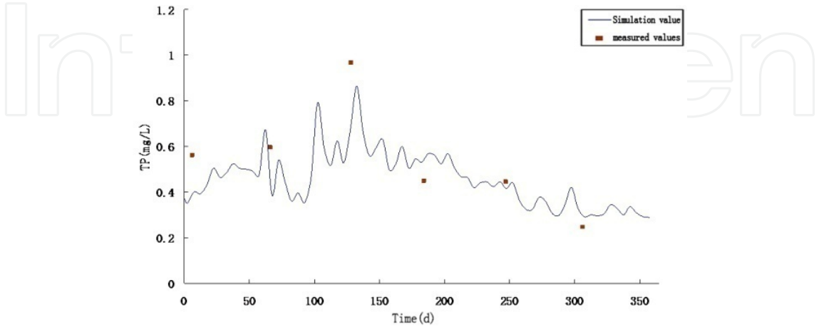
Figure 24. Verification chart for Miao Lake TP.
