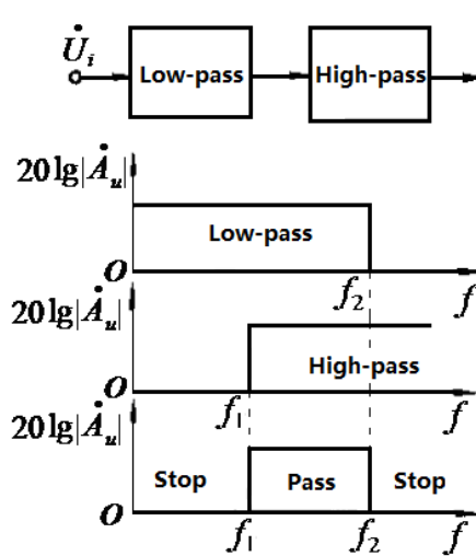
(c) Band-pass filter principle diagram
