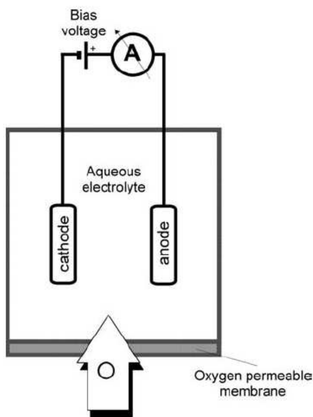
Figure 4. Sensing principle of Clark-type \text{pO}_2 sensor
