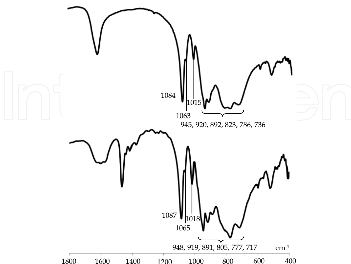
Figure 8. FTIR spectra (as KBr disks) of \text{K}_8\text{H}_2[\alpha_2\text{-P}_2\text{W}_{17}\text{MgO}_{62}]\cdot 15\text{H}_2\text{O} (Top) and [(\text{CH}_3)_2\text{NH}_2]_{7.5}\text{H}_{2.5}[\alpha_2\text{-P}_2\text{W}_{17}\text{MgO}_{62}]\cdot 6\text{H}_2\text{O} (bottom) in the range of 1800 – 400 \text{cm}^{-1} .
