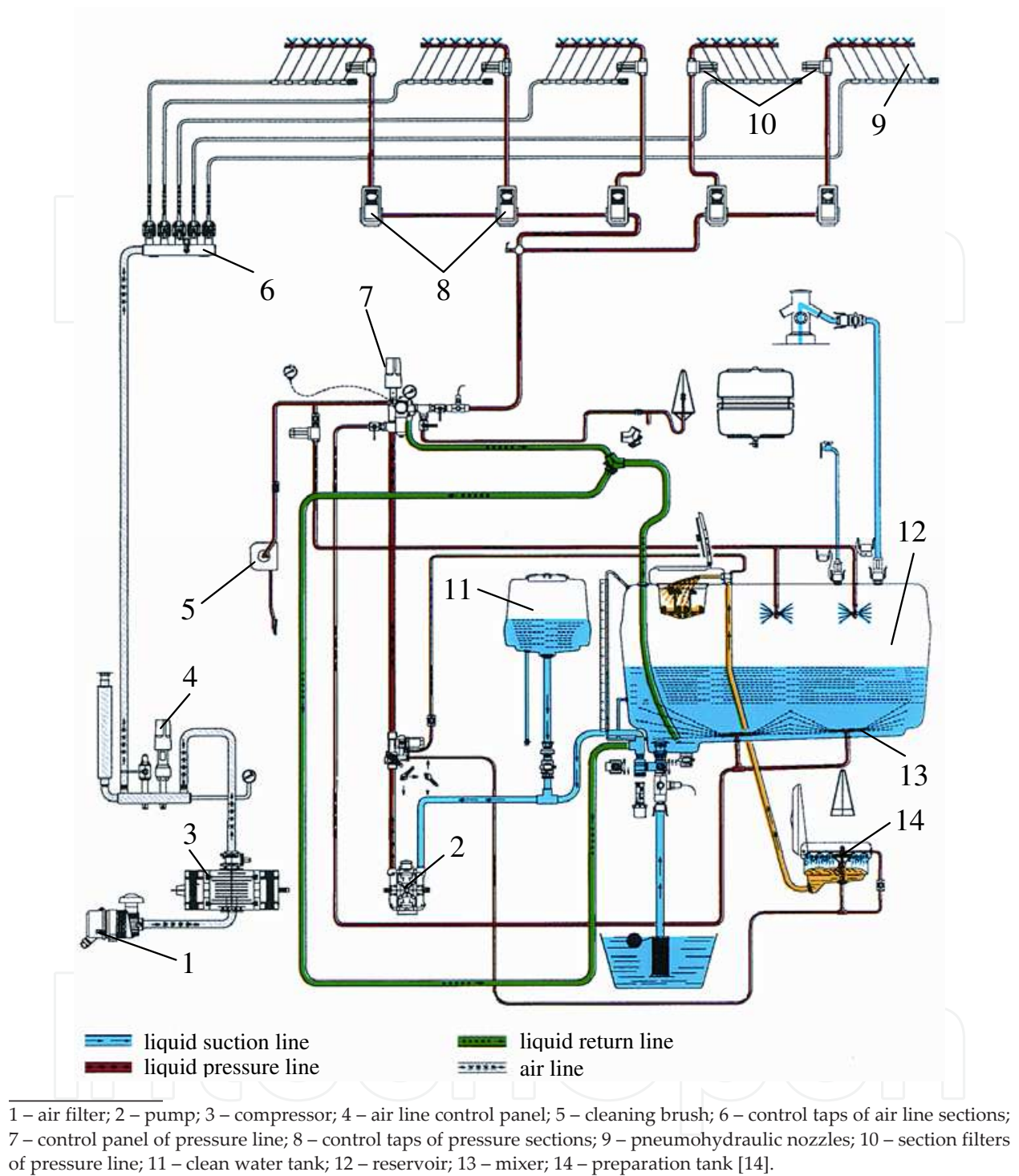
Figure 11. The scheme of a pneumohydraulic field sprayer
