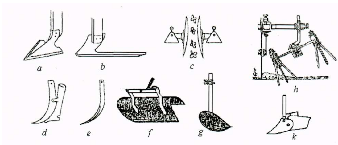
a – arrow ploughshare; b – one-side knife; c – protective plates; d – fertilizing ploughshare; e – forged ploughshare; f – protective convex; g – turning ploughshare; h – weeding rotors; i – hill-up ploughshare; j – hill-up ploughshare; k – hill-up ploughshare [26].
