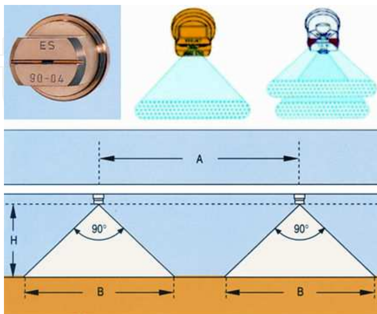
a – cleft flat-flow Lechler ES; b – cleft flat-flow TeeJet® E-type; c – two-stream TwinJet™ E-type; d – fastening scheme on sprayer beam: A – width between rows, B – area of the sprayed stripe, H – spraying height [7, 9].
