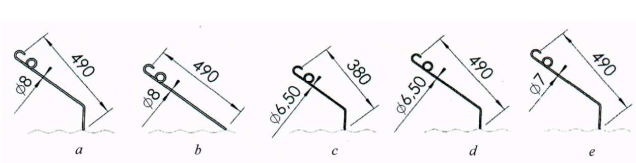
a – for heavy soil; b – for stony soil; c – for average weight soil; d – for light soil; e – for various soils (universal) [32].
