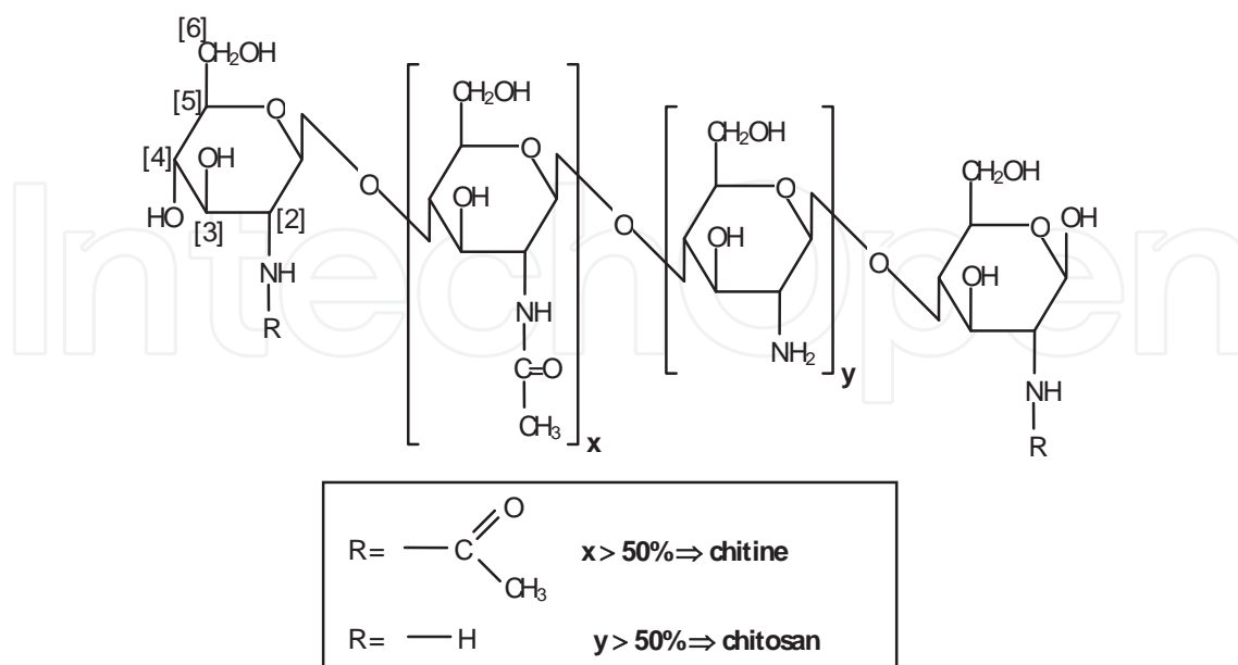
Figure 3. Chitosan - chemical structure
