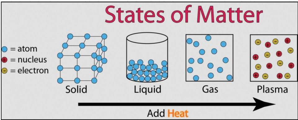
Figure 1. States of matter [90]
