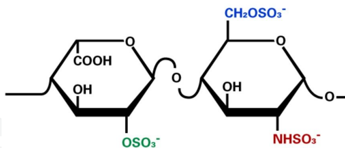
Figure 8. Chemical structure of heparin molecule [95]
