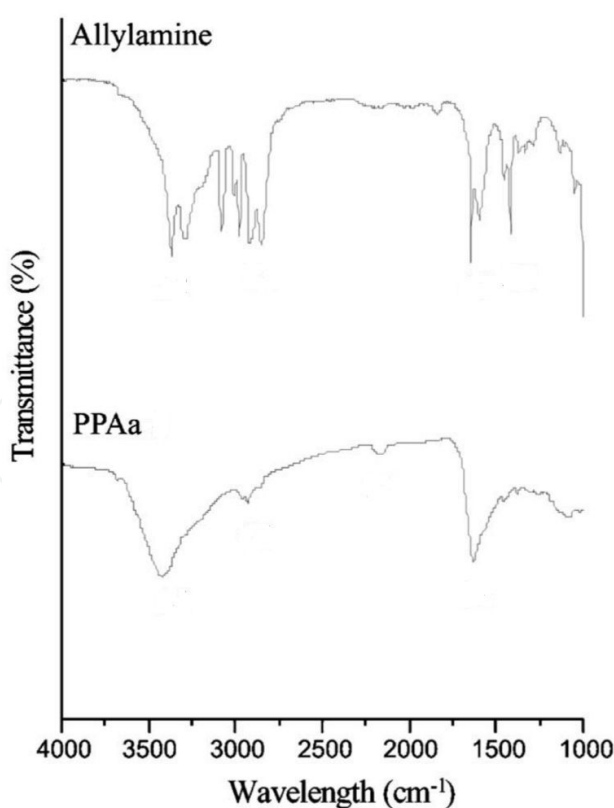
Figure 5. FTIR spectra of allylamine and PPAa [92]
