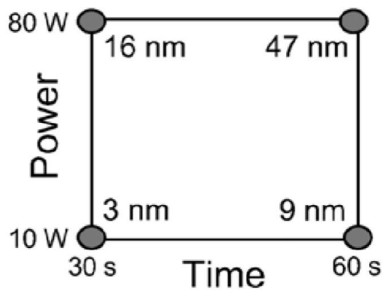
Figure 7. Square plot summarizing the influence of power and deposition time on the thickness of HApp layers [94]
