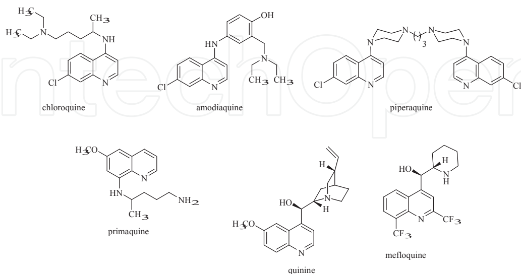
Figure 6. Structure of some quinoline alkaloids and their analogues.
