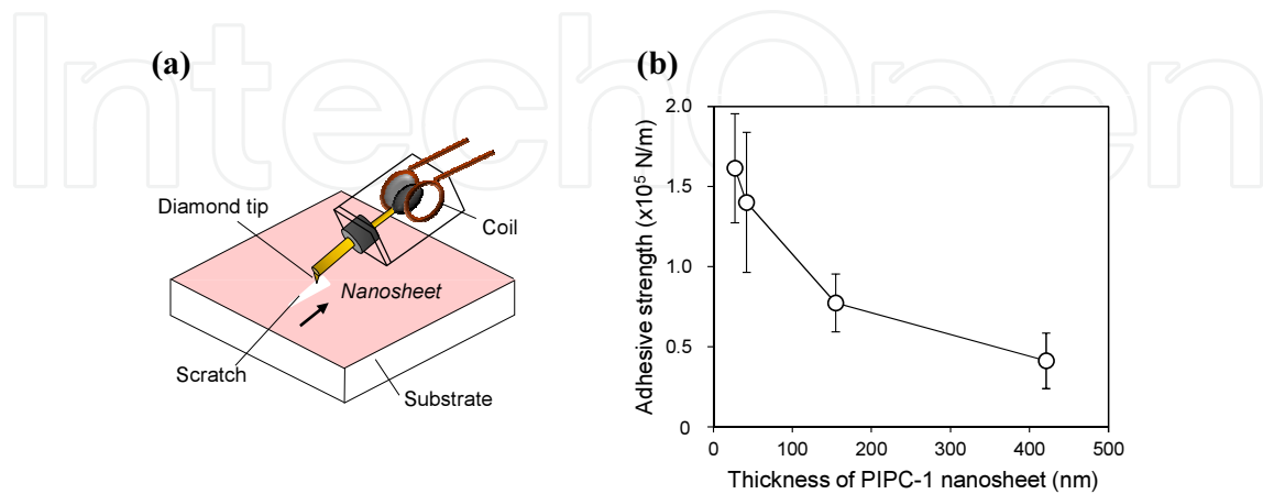
Figure 3. Adhesive strength of the PIPC-1 nanosheet. (a) Schematic image of scratch tester for thin films. (b) Correlation of adhesive strength of the PIPC-1 nanosheet with its thickness.
