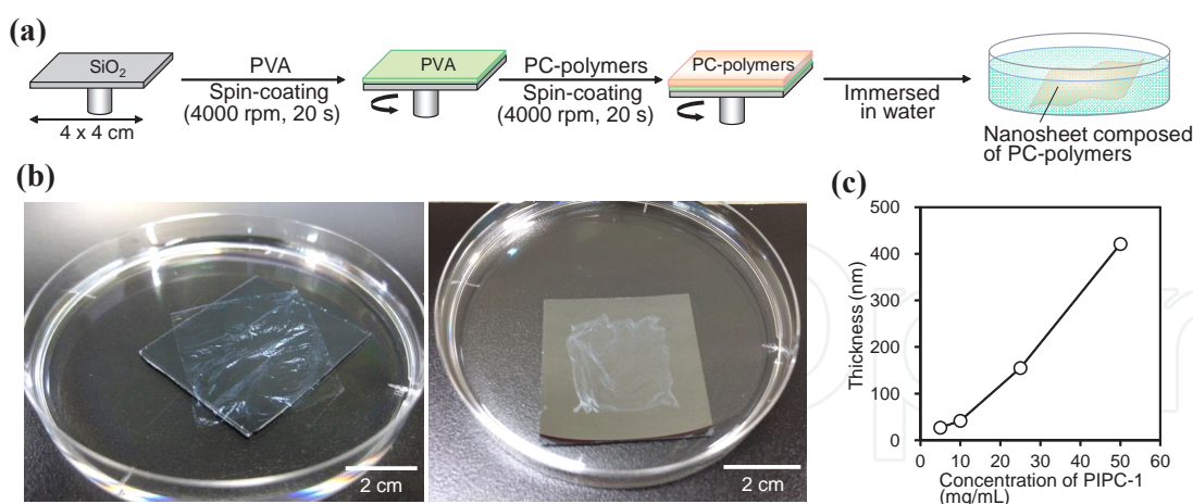
Figure 1. Fabrication of self-standing nanosheets composed of PIPC-1 and SPUPC-2. (a) Fabrication procedure of the nanosheets by spin-coating. (b) Macroscopic images of PIPC-1 (left) and SPUPC-2 (right) nanosheets suspended in water. (c) Relationship between thickness of the PIPC-1 nanosheets and concentration of PIPC-1 solution before spin coating.
