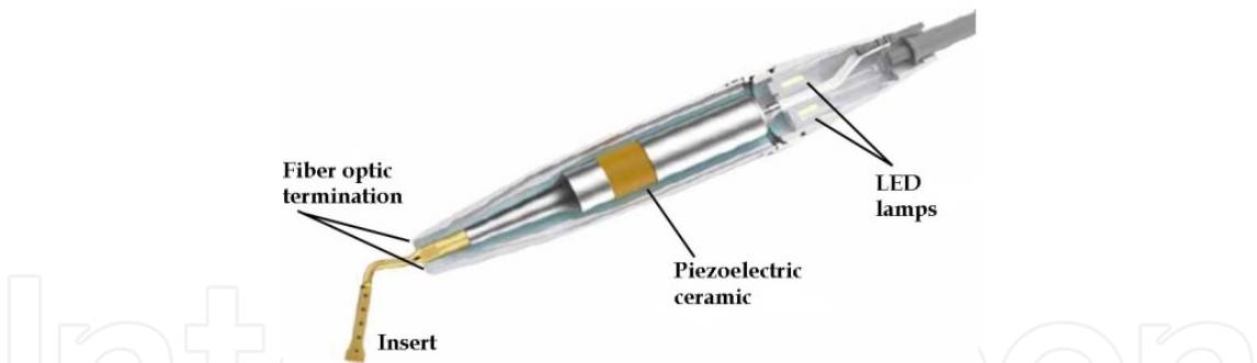
Figure 4. Piezoelectric US for surgery. Modified from Variosurg (NSK) catalogue
