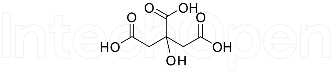
Figure 11. Citric acid
