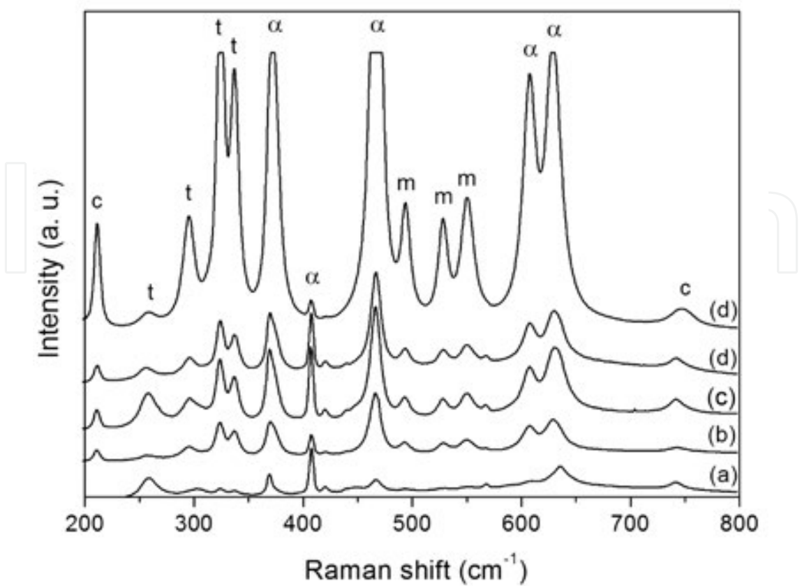
Figure 3. Micro-Raman spectra of the \text{Al}_2\text{O}_3\text{-ZrO}_2 porous ceramics at different temperatures of: (a) 1200°C, (b) 1300°C, (c) 1400°C, (d) 1500°C and (e) 1600°C. \alpha = \alpha -alumina, c = cristobalite zirconia, t = tetragonal zirconia, m = monoclinic zirconia.
