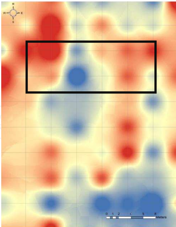
Figure 19. Difference values as calculated for MSR index
