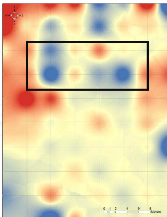
Figure 25. Difference values as calculated for ARVI index
