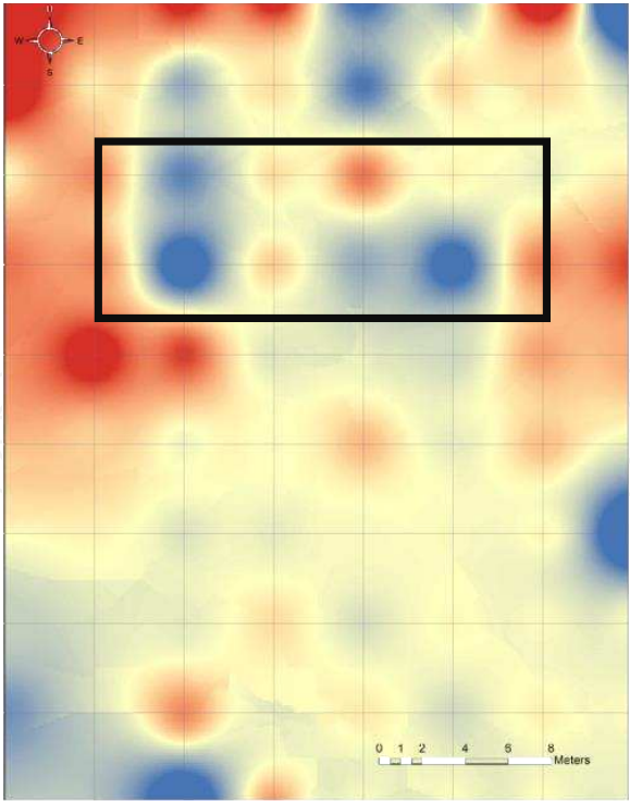
Figure 15. Difference values as calculated for SARVI index
