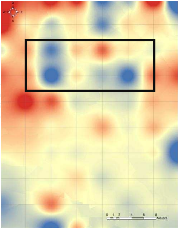
Figure 18. Difference values as calculated for NDVI index
