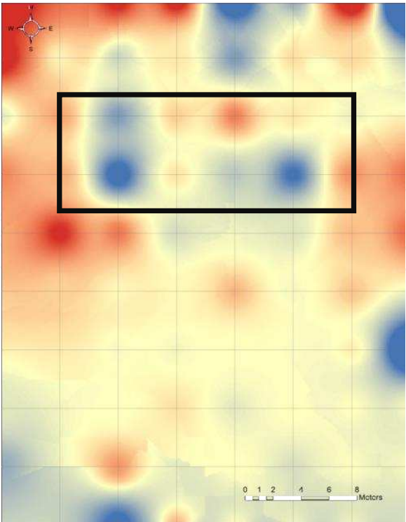
Figure 14. Difference values as calculated for SR index
