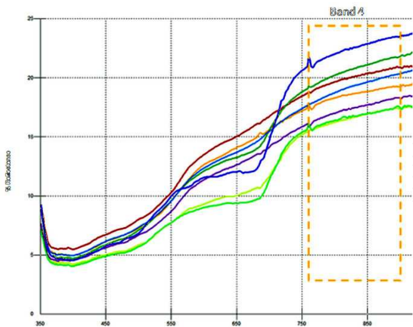
Figure 10. Spectral signatures profiles before and after the leakage event. The differences are maximized in the near infrared part of the spectrum (Band 4)
