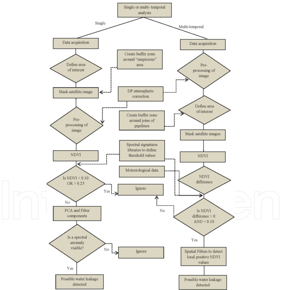
Figure 26. Methodology followed for the early warning system (Agapiou et al. 2014).
