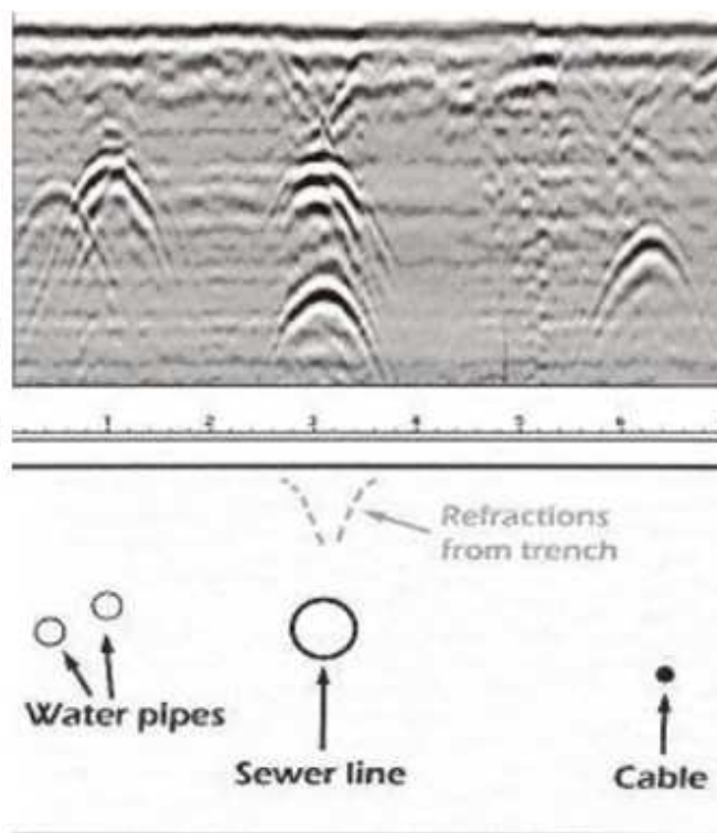
Figure 1. Reflected signals from subsurface structures
