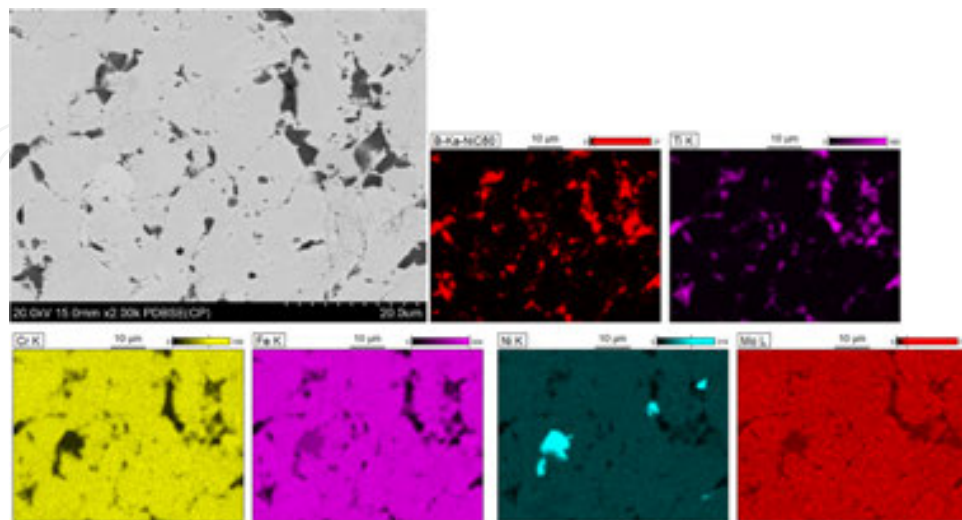
Figure 11. The microstructure of composites with 8 vol% of \text{TiB}_2 (HP-HT method, sintered at 1300^\circ\text{C} , 5 GPa) with corresponding area analysis (WDS).
