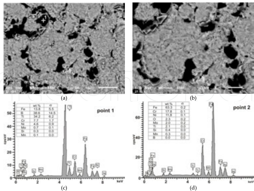
Figure 10. (a, b) The microstructure of composites with 8 vol% of TiB 2 (HP-HT method, sintered at 1300°C, 5 GPa) and (c, d) corresponding point analysis (EDS).
