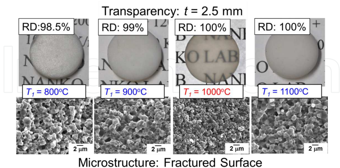
Figure 4. Appearance, fracture surface and density of polycrystalline \text{Al}_2\text{O}_3 prepared by using TS-PECS with 1 st different temperature for 60 min and 1200°C for 20 min under 100 MPa in vacuum.
