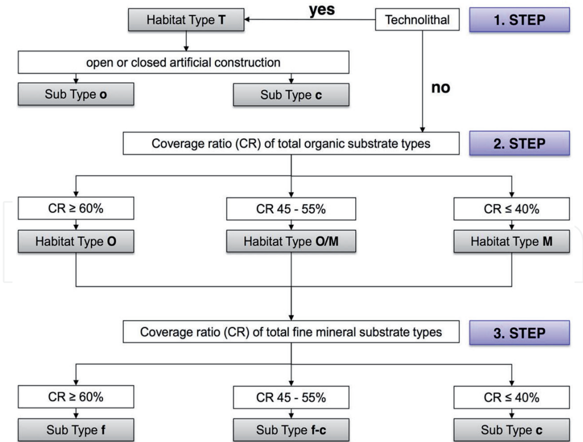
Figure 6. Decision Scheme for modelling microhabitat types of springheads. See [10].
