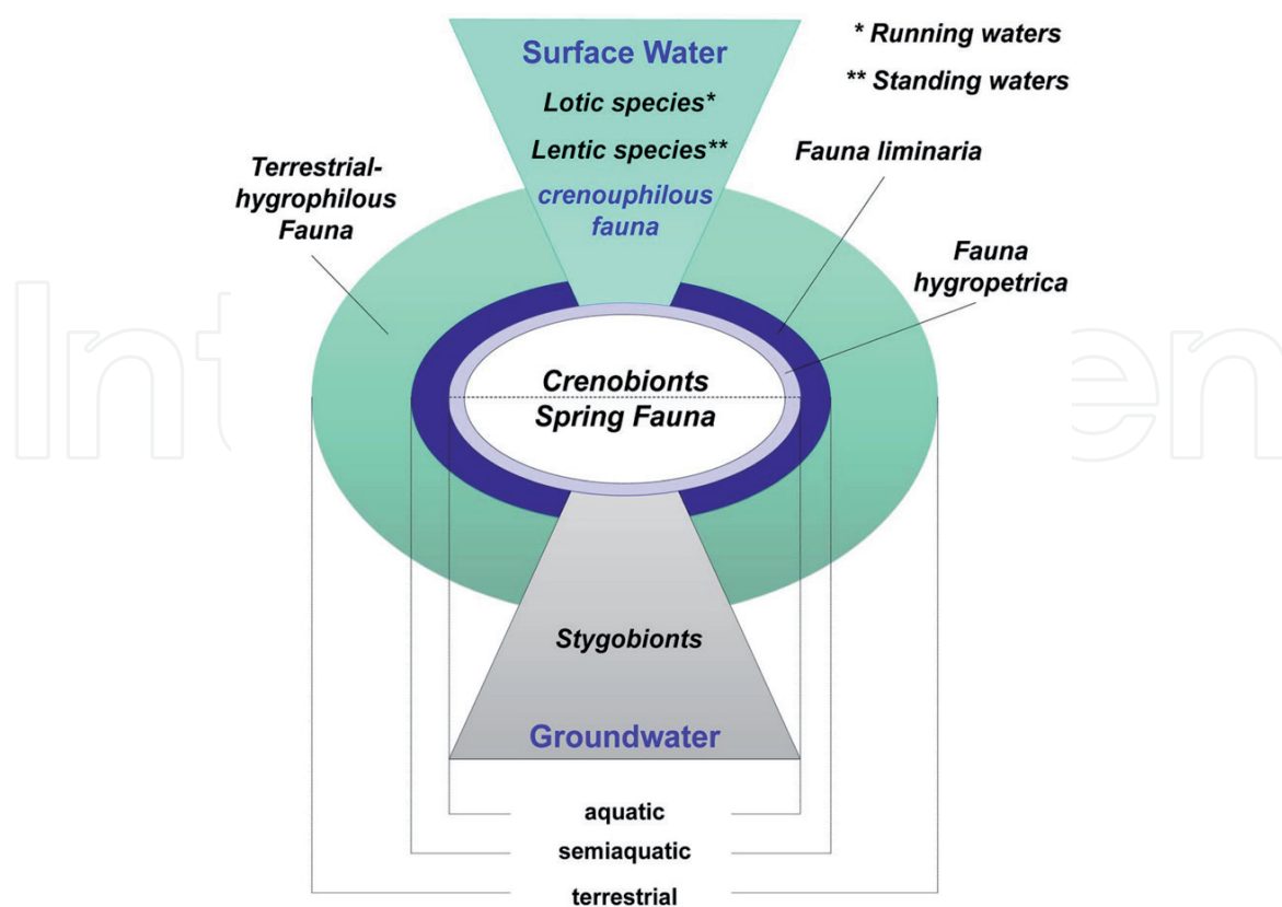
Figure 2. The eucrenal of spring ecosystems as an ecotone with its related transition fauna zones. See [10].
