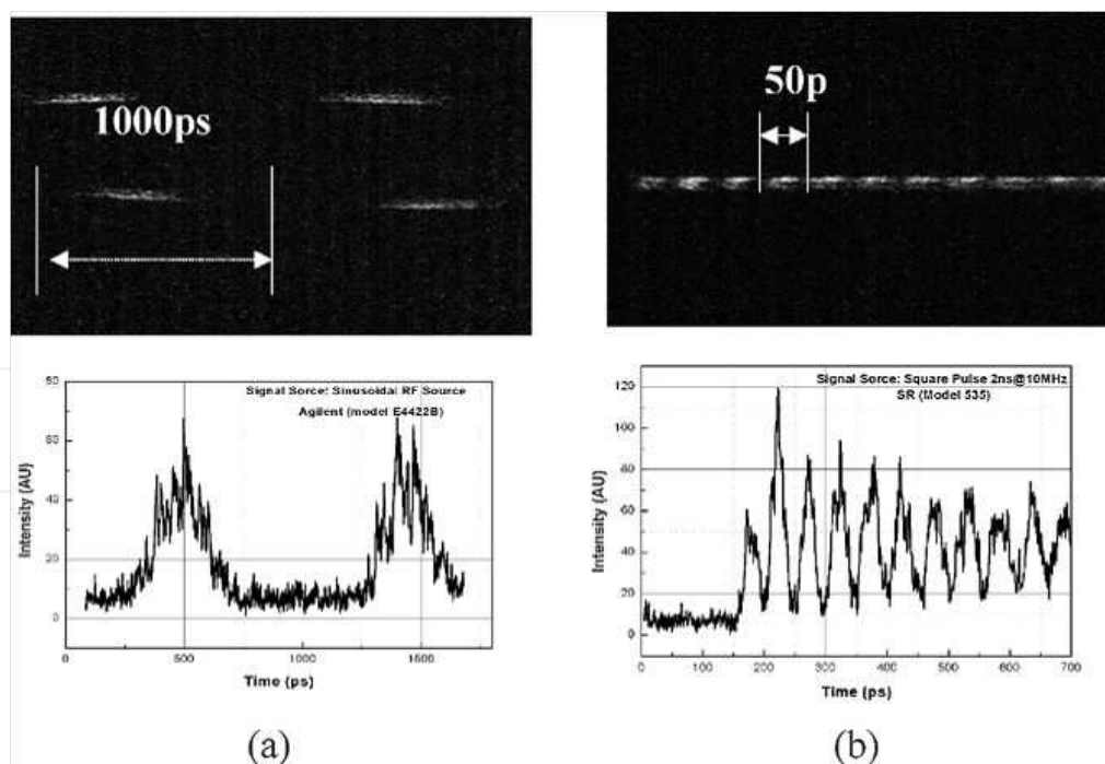
Figure 8. Light emission and intensity measurements of a test structure at: (a) 1 GHz modulation and (b) 20 GHz modulation. The spectrum of the emitted light is distributed between 430–800 nm. (After ref. [35]).
