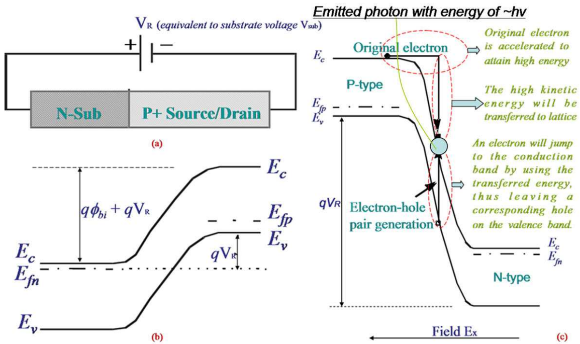
Figure 5. Energy band scheme which demonstrates current amplification due to impact ionization and depicts radiative recombination of an e - h pair giving.
