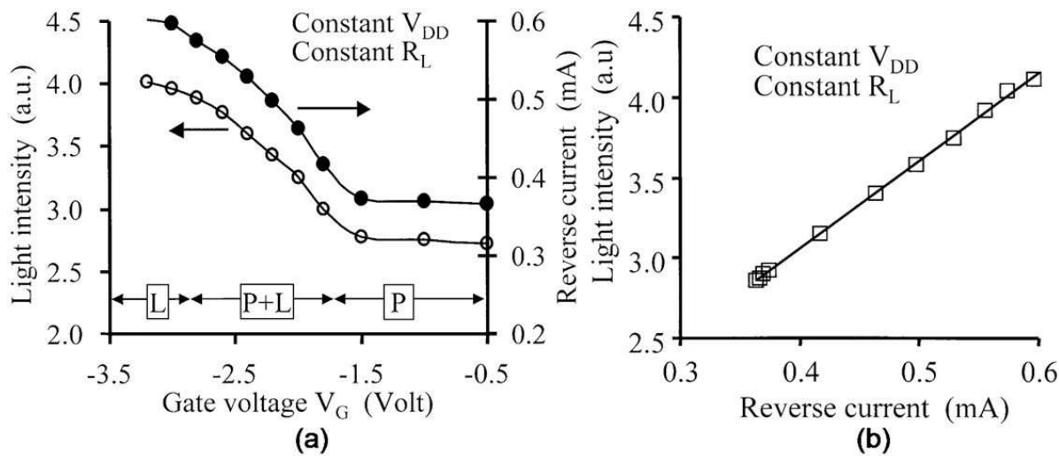
Figure 10. Light emission characteristics of the TRANSLED with constant V_{DD} . (a) Reverse current and overall light intensity, both as a function of V_G . (b) Dependence of the overall light emission on the reverse current (After ref. [40]).
