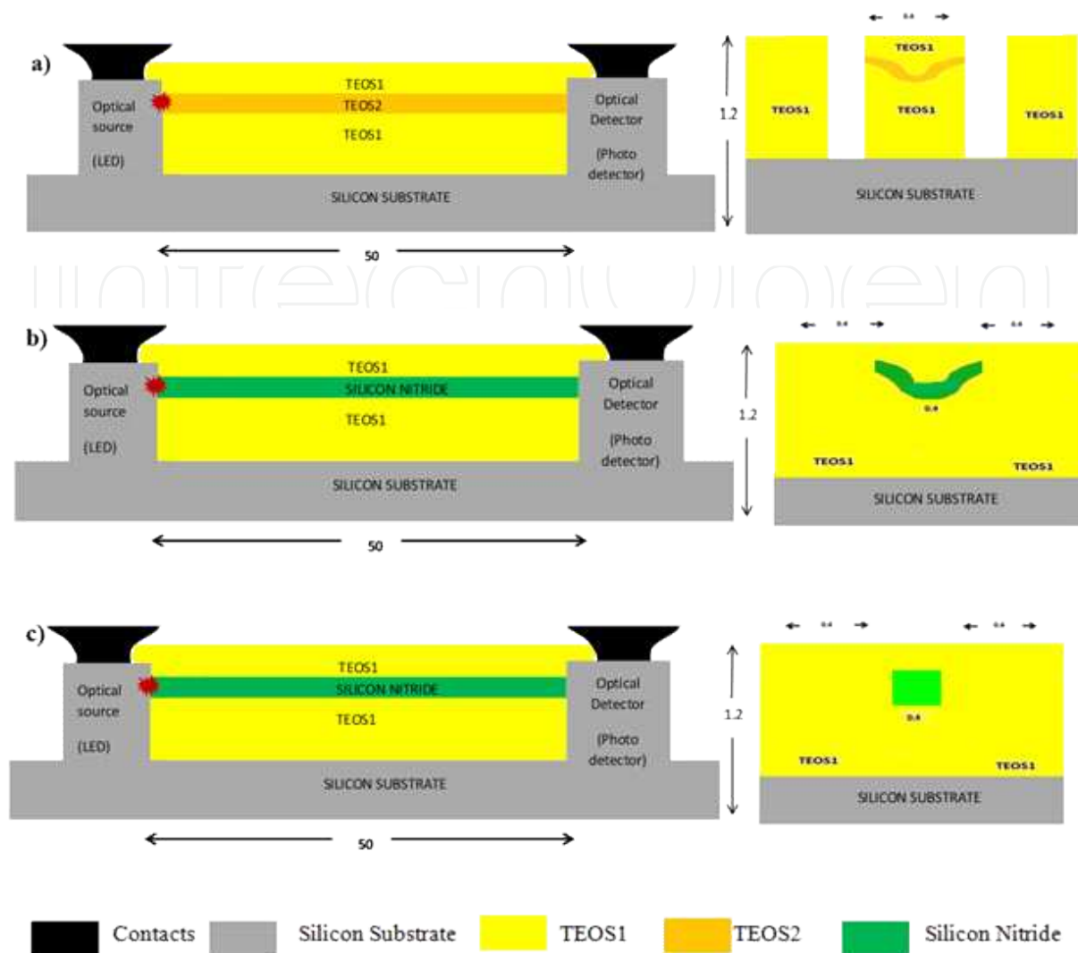
Figure 12. Schematic presentations showing the three basic designs of the waveguides of the optical links as described in this study, using Si Av LED, silicon based waveguides and Si-Ge based detectors. Cross-section layouts of the respective waveguides are given for each design. All dimensions are given in micron and not to scale.
