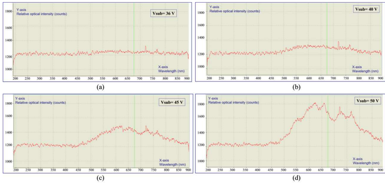
Figure 6. Output emission spectra of the Si light-emitting-device, gate is floated, V_s = V_d = 0 V. Emitting wavelength ranges from 500 nm to 850 nm in the measured range of 200 nm to 900 nm (After ref. [20]).
