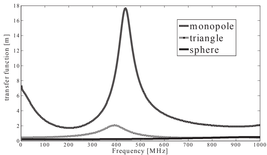
Figure 19. Transfer function of the three antennas.
