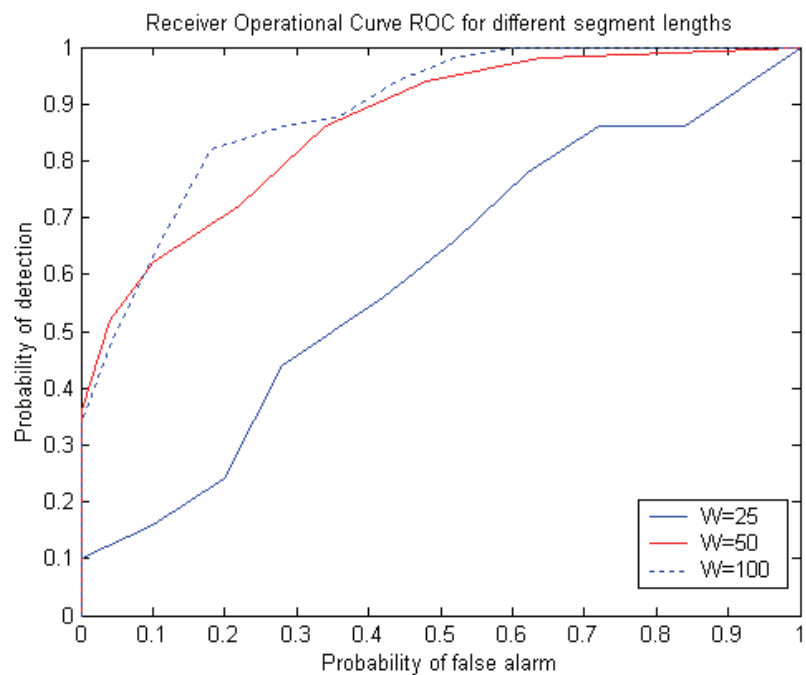
Fig. 19. Comparison between the DCS with filtration for three different window lengths.
