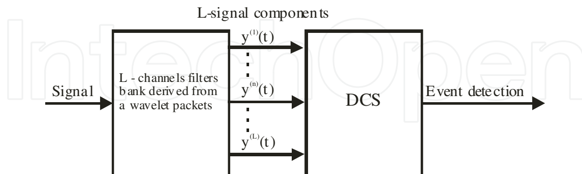
Fig. 1. Two stages algorithm for change detection ( L is the number of filters used).
