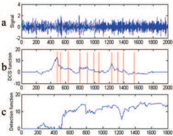
Fig. 14. Application of the DCS on a signal with frequency change. a) Original signal. b) DCS function. c) Detection function g(t) .
