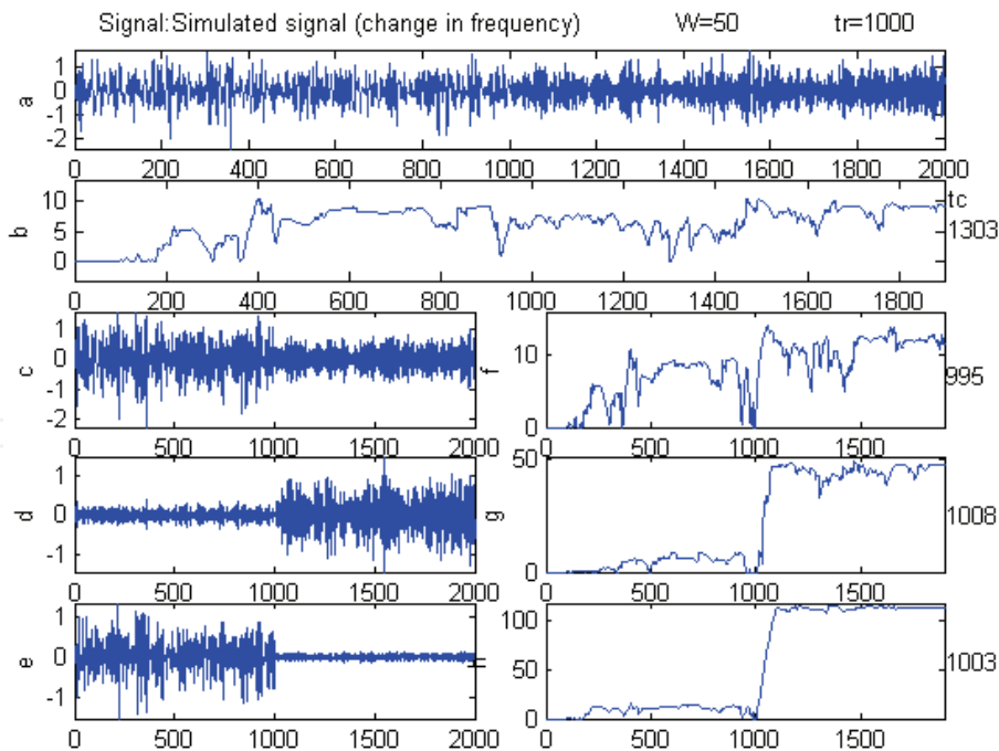
Fig. 15. Results after the decomposition. At left: decomposition of the signal into 3 components. At right: the detection functions of each component. a) Original signal presenting frequency change at 1000 T.U. b) DCS applied directly on the original signal. c) d) e) Decomposition using filters bank derived from the 'Haar' wavelet packet. f) g) h) Detection functions applied on the filtered signals (c, d, e).
