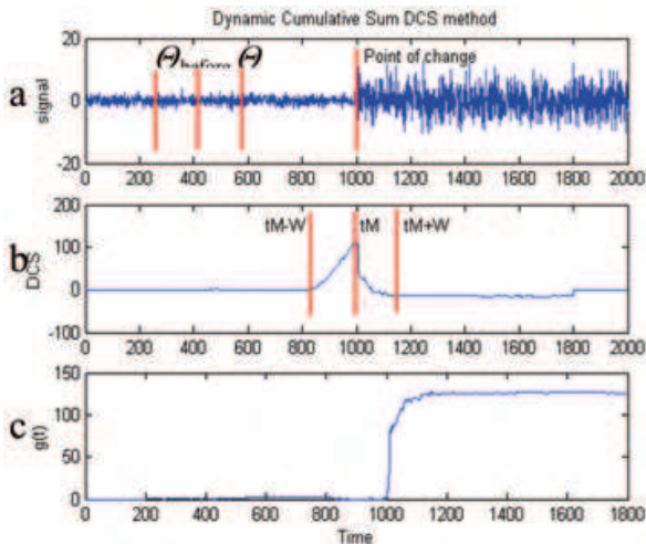
Fig. 13. Application of the DCS on a signal of abrupt change. a) Original signal. b) DCS function. c) Detection function g(t) .
