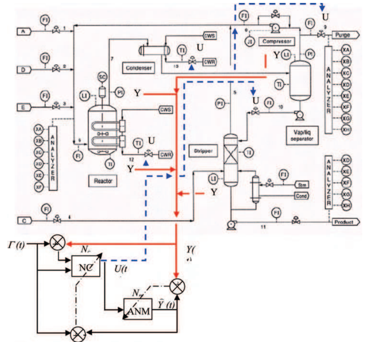
Fig. 20. Tennessee Eastman Challenge Process and robust adaptive neural networks controller (Leclercq et al., 2005), (Zerkaoui et al, 2007).
