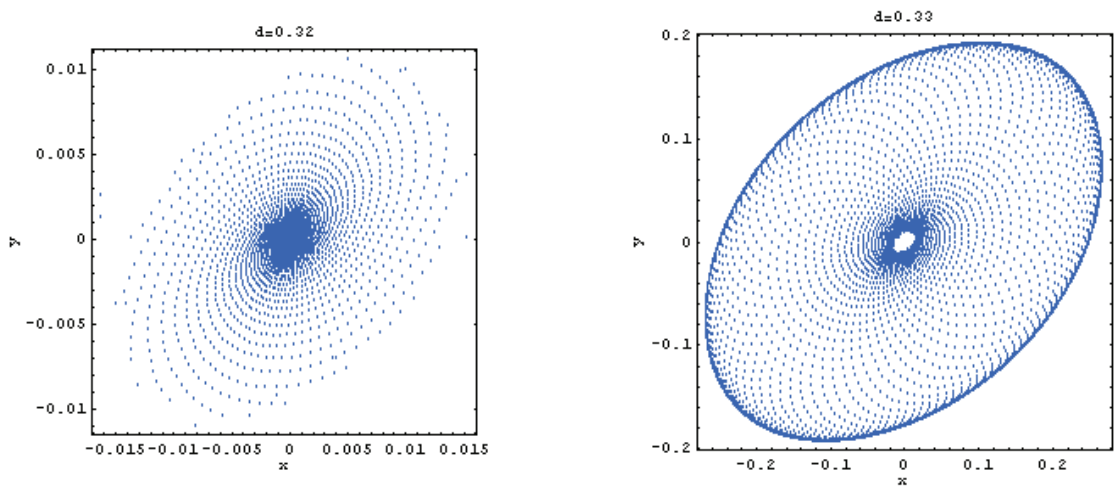
Fig. 4. Supercritical Neimark-Sacker bifurcation at \delta = 0.324255 . For \delta = 0.32 , the null solution is asymptotically stable, and the trajectory converges to the origin. For b = 0.33 , an asymptotically stable cycle (1-torus) is present, and the trajectory converges to this cycle.
