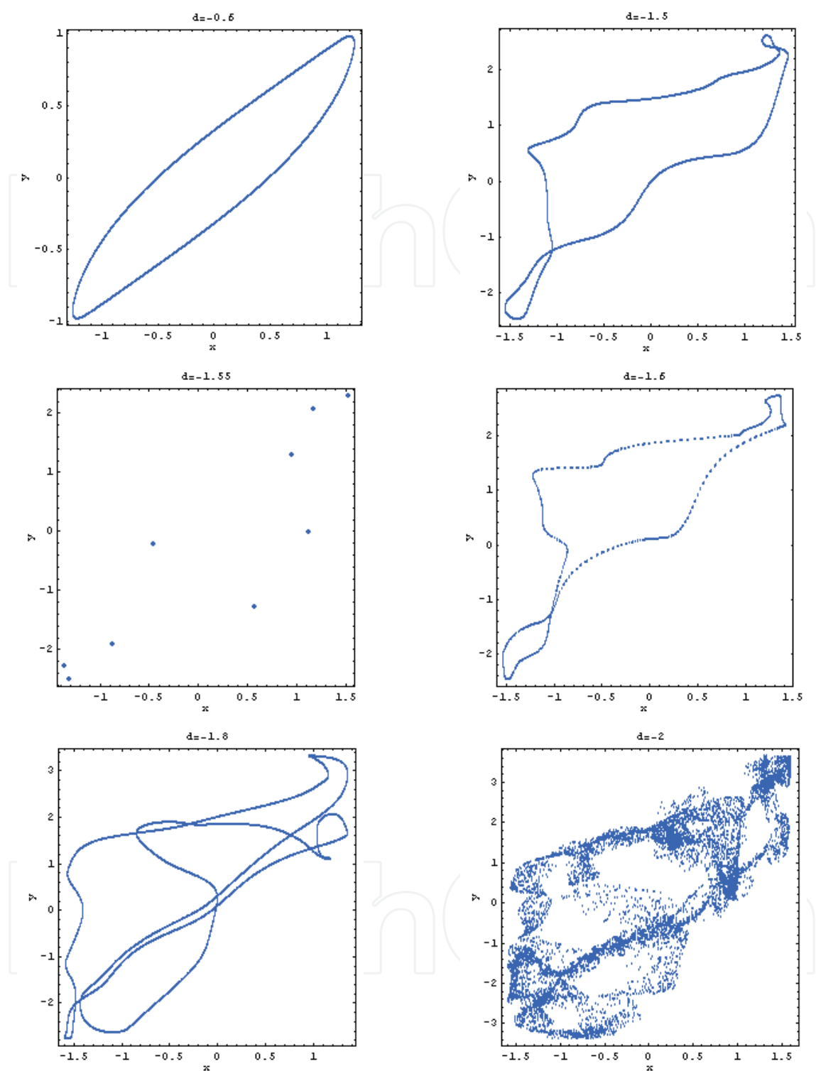
Fig. 7: Phase portraits for various values of \delta \in (-2.5, 0) , at the first step towards chaos. The route towards chaos passes through several stages: \delta = -0.6 , \delta = -1.5 : 1-toruses (LLCE = 0); \delta = -1.55 : stable period-9 orbit (LLCE < 0); \delta = -1.6 : 1-torus (LLCE = 0); \delta = -1.8 : 2-torus (LLCE = 0), \delta = -2 : strange attractor (LLCE \approx 0). For each plot, considering the initial conditions (x_0, y_0) = (0.01, 0.01) , the first 10^6 iterations of system (10) have been dropped, and the next 10^4 iterations have been plotted.
