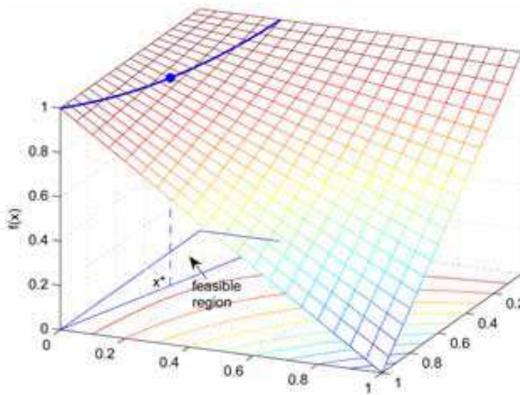
Figure 6. Isometric view of the objective function and constraints in Example 3. Reprint of Fig. 9.1 in (Hu, 2007).
