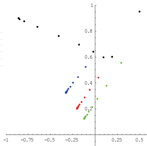
Fig. 3. Points of \{(f_- f_+)^n(p) \mid 11 \geq n \geq 1\} , where p = (0.5, 0.95) are plotted over the left-hand pane of Fig. 2, which shows that the points do not stay in D_0 . The points start from p and converge at around (-0.8595, 0.8984) .
