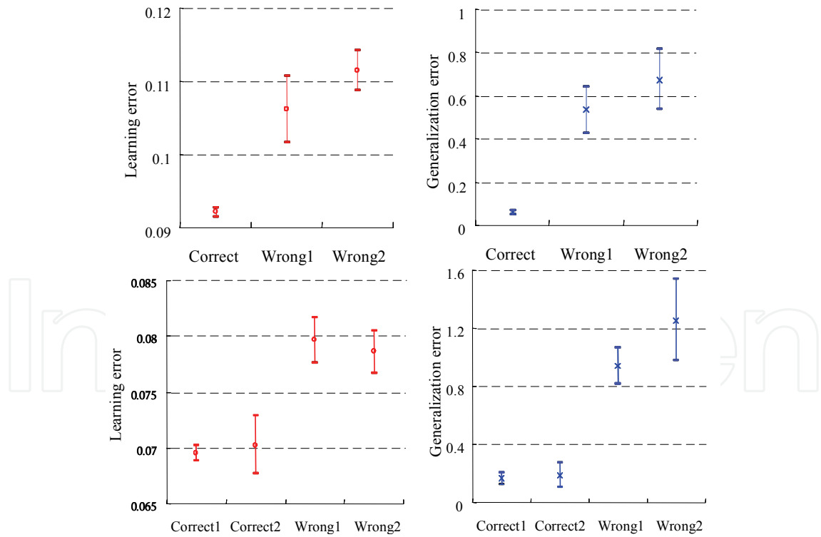
Fig. 5. Top two figures. L = 6, D = 2, Nc = 3, and N = 60. On the horizontal axis, Correct is \{a_1,a_2\}, \{b_1,b_2\}, \{t\} , Wrong1 is \{a_1\}, \{a_2,b_1,b_2\}, \{t\} and Wrong2 is \{a_1,b_1\}, \{a_2,b_2\}, \{t\} . Bottom two figures. L = 8, D = 4, Nc = 4, and N = 60. On the horizontal axis, Correct1 is \{a_1,a_2,a_3,a_4\}, \{b_1,b_2\}, \{b_3,b_4\}, \{t\} , Correct2 is \{a_1,a_2,a_3,a_4\}, \{b_1,b_2,b_3\}, \{b_4\}, \{t\} , Wrong1 is \{a_1,a_2,b_1\}, \{a_3,a_4,b_2\}, \{b_3,b_4\}, \{t\} and Wrong2 is \{a_1,a_2,b_3,b_4\}, \{a_1,b_1\}, \{a_2,b_2\}, \{t\}
