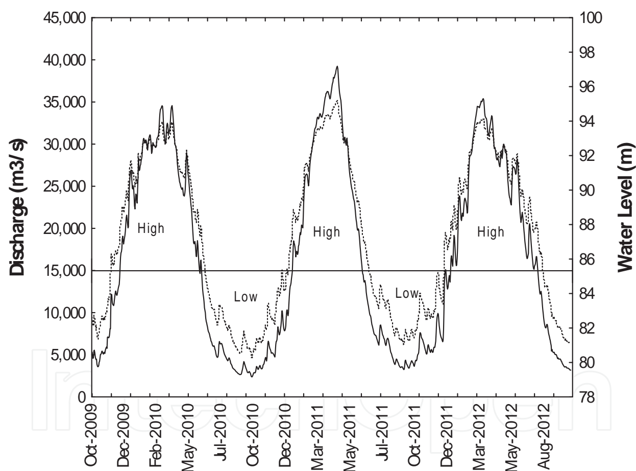
Figure 3. The hydrological cycle of the Madeira River Basin obtained at the Hydrological Station of Abunã, at the up-river of the study area (discharge- continuous line; water level- dotted line).
